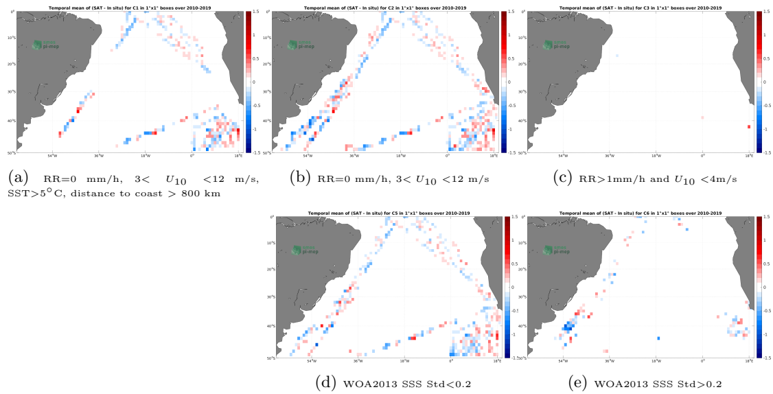
Figure 12: Temporal mean gridded over spatial boxes of size 1^\circ \times 1^\circ of \Delta\text{SSS} (SMOS SSS L3 v332 - 9 Days (CATDS-CPDC) - TSG (Polarstern)) for 5 different subdatasets corresponding to:RR=0 mm/h, 3 < U_{10} < 12 m/s, SST >5^\circ\text{C} , distance to coast > 800 km (a), RR=0 mm/h, 3 < U_{10} < 12 m/s (b), RR >1 mm/h and U_{10} < 4 m/s (c), WOA2013 SSS Std <0.2 (d), WOA2013 SSS Std >0.2 (e).
