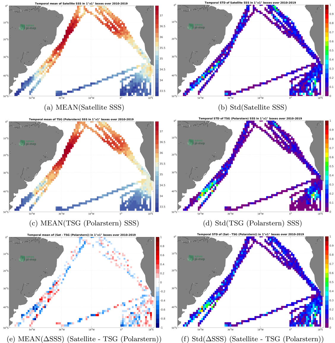
Figure 6: Temporal mean (left) and Std (right) of SSS from SMOS SSS L3 v332 - 9 Days (CATDS-CPDC) (top), TSG (Polarstern) (middle), and of \Delta SSS (Satellite - TSG (Polarstern)). Only match-up pairs are used to generate these maps.
