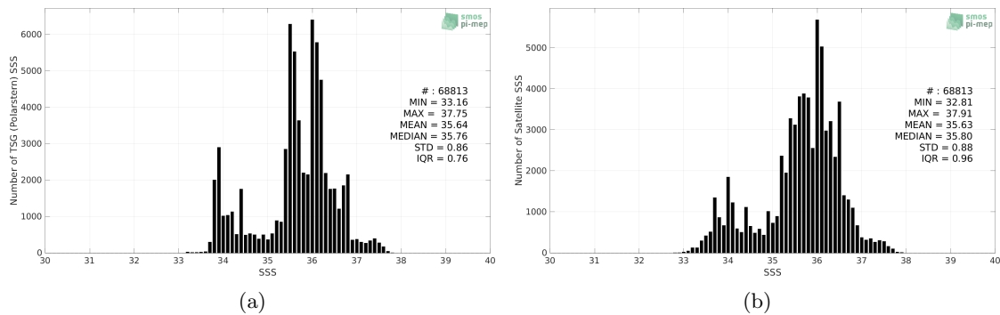
Figure 2: Histograms of SSS from TSG (Polarstern) (a) and SMOS SSS L3 v332 - 9 Days (CATDS-CPDC) (b) considering all match-up pairs per bins of 0.1 over the South Atlantic Ocean Pi-MEP region and for the full satellite product period.
