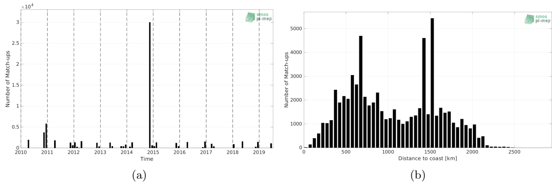
Figure 1: Number of match-ups between TSG (Polarstern) and SMOS SSS L3 v332 - 9 Days (CATDS-CPDC) SSS as a function of time (a) and as function of the distance to coast (b) over the South Atlantic Ocean Pi-MEP region and for the full satellite product period.
