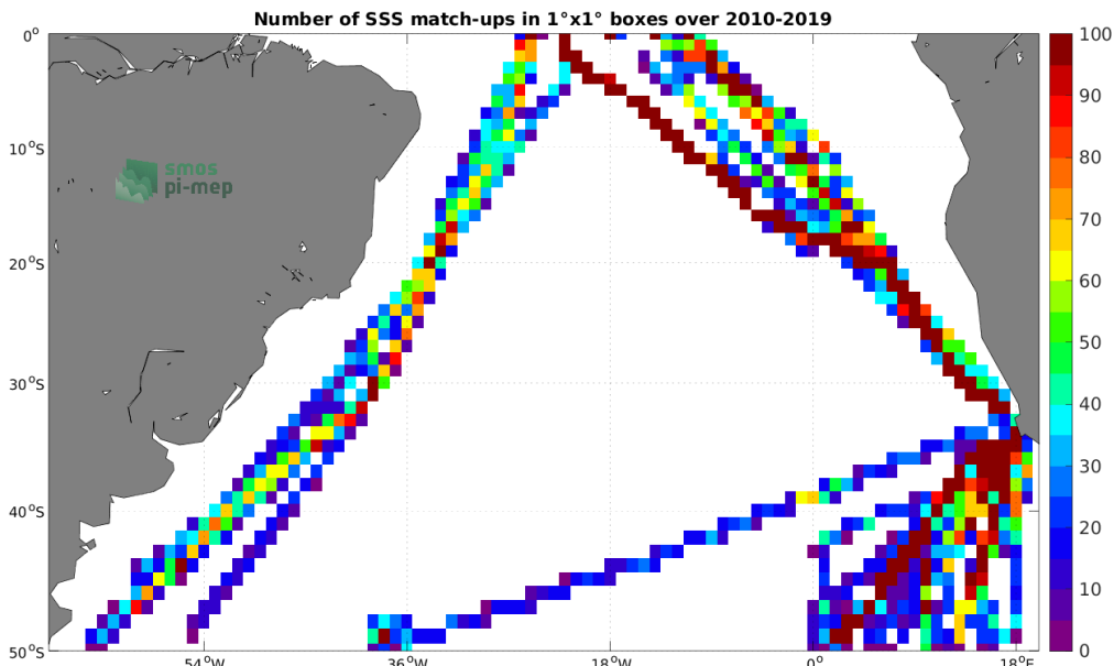
Figure 4: Number of SSS match-ups between TSG (Polarstern) SSS and the SMOS SSS L3 v332 - 9 Days (CATDS-CPDC) SSS product for the South Atlantic Ocean Pi-MEP region over 1^\circ \times 1^\circ boxes and for the full satellite product period.
