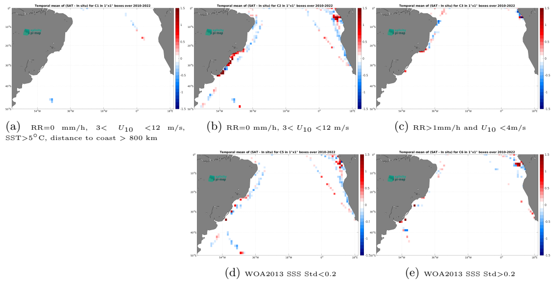
Figure 12: Temporal mean gridded over spatial boxes of size 1^\circ \times 1^\circ of \Delta SSS (SMOS SSS L3 v332 - 9 Days (CATDS-CPDC) - TSG (LEGOS-DM)) for 5 different subdatasets corresponding to:RR=0 mm/h, 3 < U_{10} < 12 m/s, SST >5^\circ\text{C} , distance to coast > 800 km (a), RR=0 mm/h, 3 < U_{10} < 12 m/s (b), RR >1 mm/h and U_{10} < 4 m/s (c), WOA2013 SSS Std <0.2 (d), WOA2013 SSS Std >0.2 (e).
