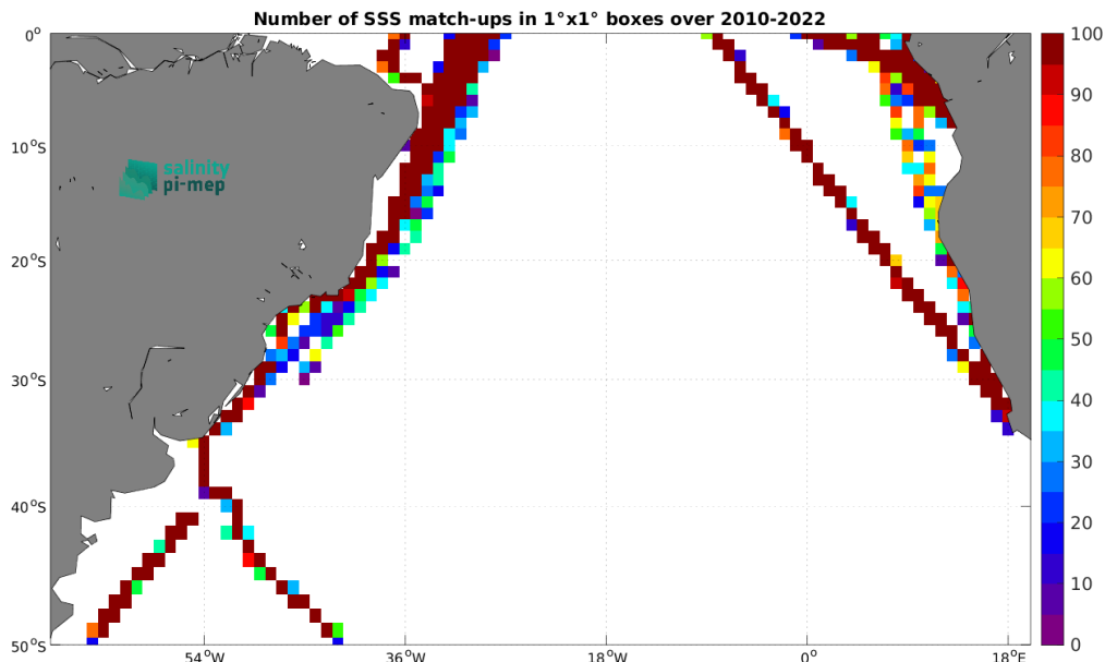
Figure 4: Number of SSS match-ups between TSG (LEGOS-DM) SSS and the SMOS SSS L3 v332 - 9 Days (CATDS-CPDC) SSS product for the South Atlantic Ocean Pi-MEP region over 1^\circ \times 1^\circ boxes and for the full satellite product period.
