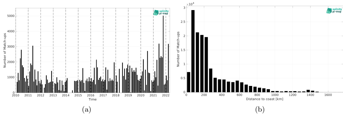
Figure 1: Number of match-ups between TSG (LEGOS-DM) and SMOS SSS L3 v332 - 9 Days (CATDS-CPDC) SSS as a function of time (a) and as function of the distance to coast (b) over the South Atlantic Ocean Pi-MEP region and for the full satellite product period.
