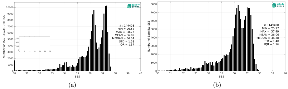
Figure 2: Histograms of SSS from TSG (LEGOS-DM) (a) and SMOS SSS L3 v332 - 9 Days (CATDS-CPDC) (b) considering all match-up pairs per bins of 0.1 over the South Atlantic Ocean Pi-MEP region and for the full satellite product period.
