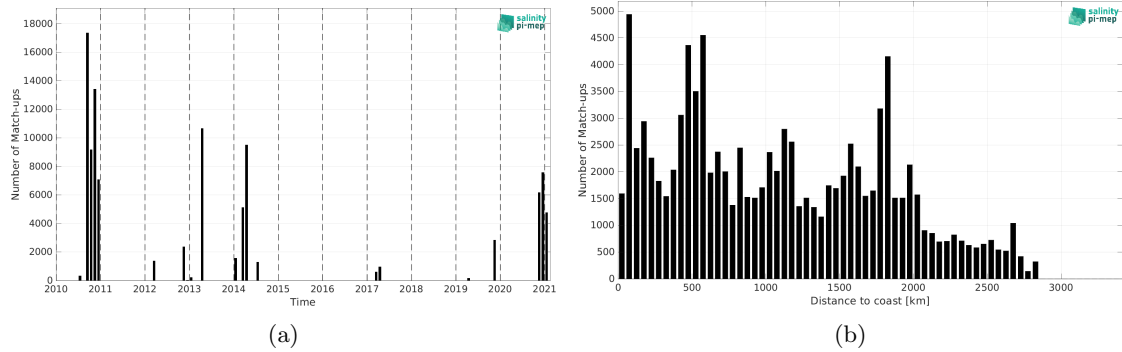
Figure 2: Number of match-ups between TSG (GOSUD-Sailing-ship) and SMOS SSS L3 v332 - 9 Days (CATDS-CPDC) SSS as a function of time (a) and as function of the distance to coast (b) over the South Atlantic Ocean Pi-MEP region and for the full satellite product period.
