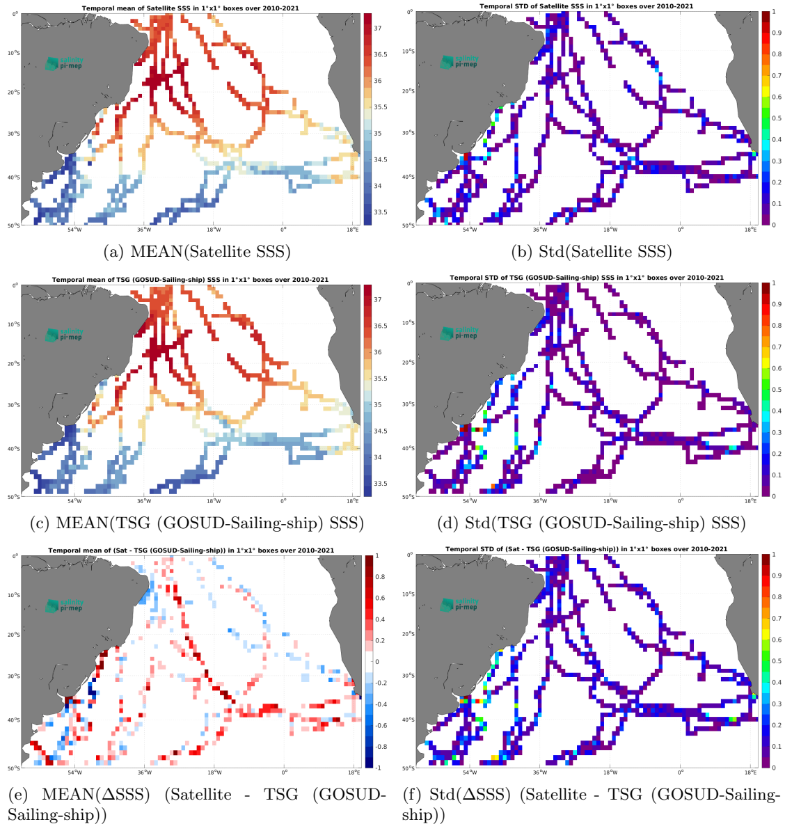
Figure 7: Temporal mean (left) and Std (right) of SSS from SMOS SSS L3 v332 - 9 Days (CATDS-CPDC) (top), TSG (GOSUD-Sailing-ship) (middle), and of \Delta SSS (Satellite - TSG (GOSUD-Sailing-ship)). Only match-up pairs are used to generate these maps.
