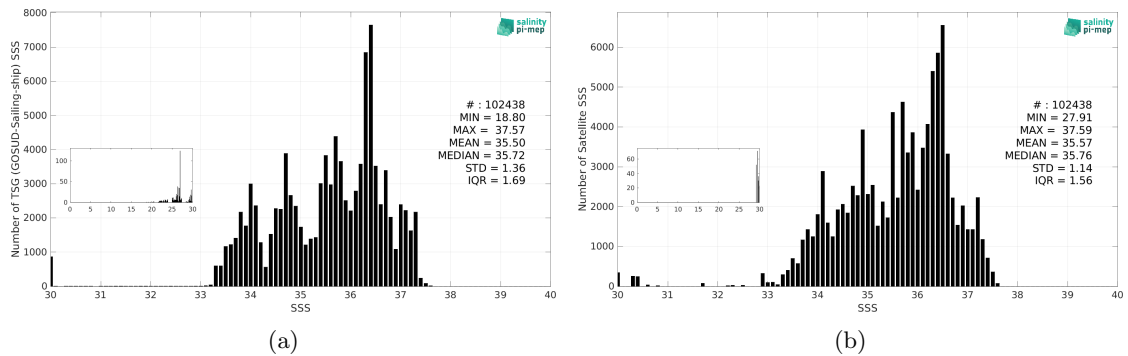
Figure 3: Histograms of SSS from TSG (GOSUD-Sailing-ship) (a) and SMOS SSS L3 v332 - 9 Days (CATDS-CPDC) (b) considering all match-up pairs per bins of 0.1 over the South Atlantic Ocean Pi-MEP region and for the full satellite product period.
