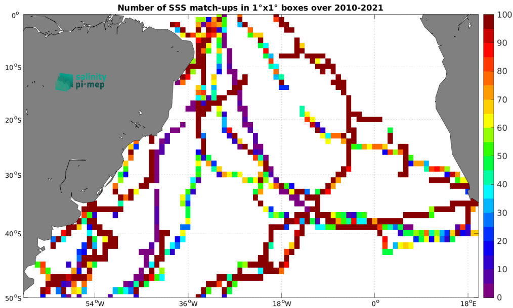
Figure 5: Number of SSS match-ups between TSG (GOSUD-Sailing-ship) SSS and the SMOS SSS L3 v332 - 9 Days (CATDS-CPDC) SSS product for the South Atlantic Ocean Pi-MEP region over 1^\circ \times 1^\circ boxes and for the full satellite product period.
