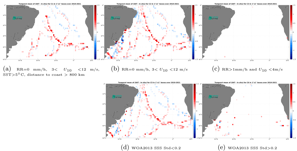
Figure 14: Temporal mean gridded over spatial boxes of size 1^\circ \times 1^\circ of \Delta\text{SSS} (SMOS SSS L3 v332 - 9 Days (CATDS-CPDC) - TSG (GOSUD-Sailing-ship)) for 5 different subdatasets corresponding to:RR=0 mm/h, 3 < U_{10} < 12 m/s, SST >5^\circ\text{C} , distance to coast > 800 km (a), RR=0 mm/h, 3 < U_{10} < 12 m/s (b), RR >1 mm/h and U_{10} < 4 m/s (c), WOA2013 SSS Std <0.2 (d), WOA2013 SSS Std >0.2 (e).
