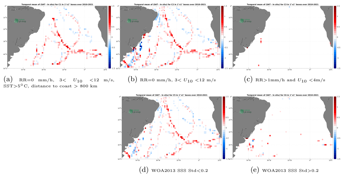
Figure 12: Temporal mean gridded over spatial boxes of size 1^\circ \times 1^\circ of \Delta SSS (SMOS SSS L3 v332 - 9 Days (CATDS-CPDC) - TSG (GOSUD-Sailing-ship)) for 5 different subdatasets corresponding to:RR=0 mm/h, 3 < U_{10} < 12 m/s, SST>5°C, distance to coast > 800 km (a), RR=0 mm/h, 3 < U_{10} < 12 m/s (b), RR>1mm/h and U_{10} < 4 m/s (c), WOA2013 SSS Std<0.2 (d), WOA2013 SSS Std>0.2 (e).
