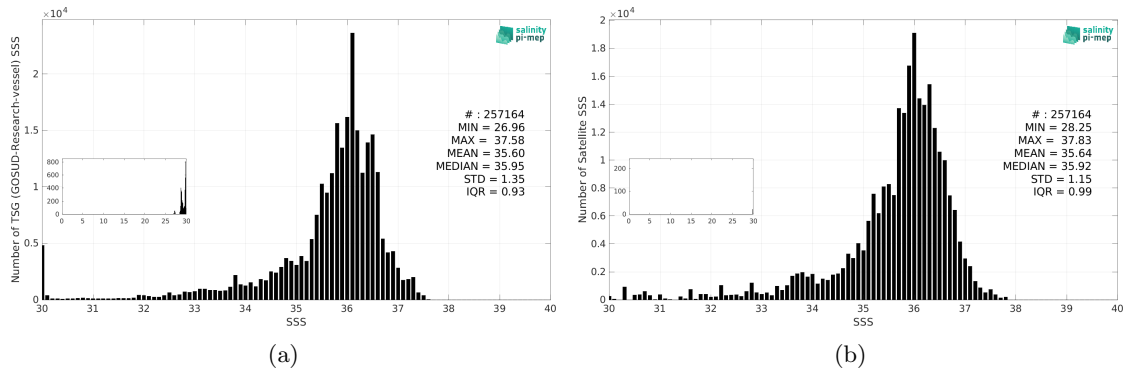
Figure 3: Histograms of SSS from TSG (GOSUD-Research-vessel) (a) and SMOS SSS L3 v332 - 9 Days (CATDS-CPDC) (b) considering all match-up pairs per bins of 0.1 over the South Atlantic Ocean Pi-MEP region and for the full satellite product period.
