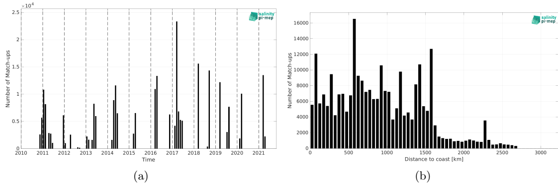
Figure 2: Number of match-ups between TSG (GOSUD-Research-vessel) and SMOS SSS L3 v332 - 9 Days (CATDS-CPDC) SSS as a function of time (a) and as function of the distance to coast (b) over the South Atlantic Ocean Pi-MEP region and for the full satellite product period.
