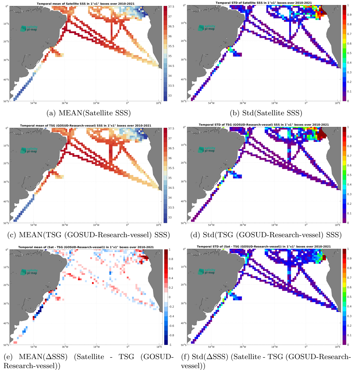
Figure 7: Temporal mean (left) and Std (right) of SSS from SMOS SSS L3 v332 - 9 Days (CATDS-CPDC) (top), TSG (GOSUD-Research-vessel) (middle), and of \Delta SSS (Satellite - TSG (GOSUD-Research-vessel)). Only match-up pairs are used to generate these maps.
