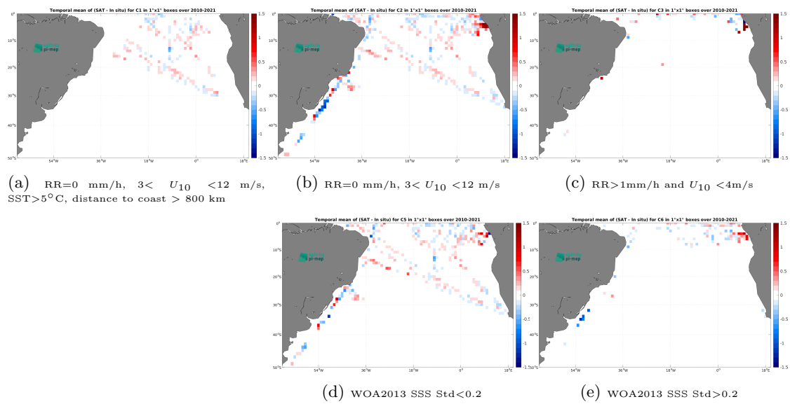
Figure 14: Temporal mean gridded over spatial boxes of size 1^\circ \times 1^\circ of \Delta\text{SSS} (SMOS SSS L3 v332 - 9 Days (CATDS-CPDC) - TSG (GOSUD-Research-vessel)) for 5 different subdatasets corresponding to:RR=0 mm/h, 3 < U_{10} < 12 m/s, SST >5^\circ\text{C} , distance to coast > 800 km (a), RR=0 mm/h, 3 < U_{10} < 12 m/s (b), RR >1 mm/h and U_{10} < 4 m/s (c), WOA2013 SSS Std <0.2 (d), WOA2013 SSS Std >0.2 (e).
