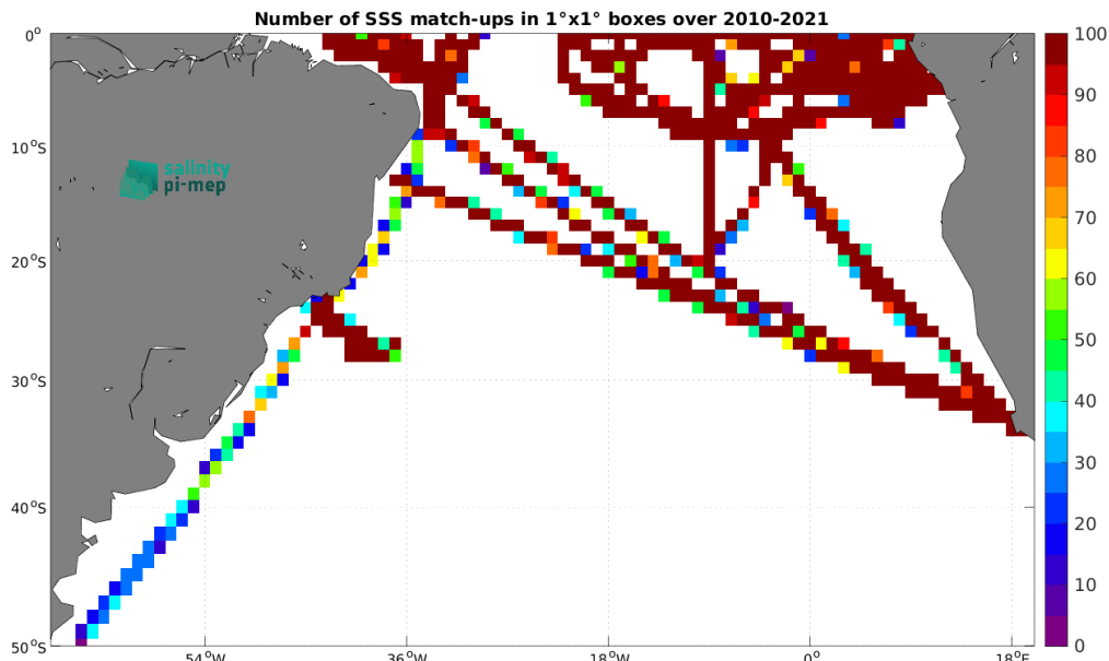
Figure 5: Number of SSS match-ups between TSG (GOSUD-Research-vessel) SSS and the SMOS SSS L3 v332 - 9 Days (CATDS-CPDC) SSS product for the South Atlantic Ocean Pi-MEP region over 1^\circ \times 1^\circ boxes and for the full satellite product period.
