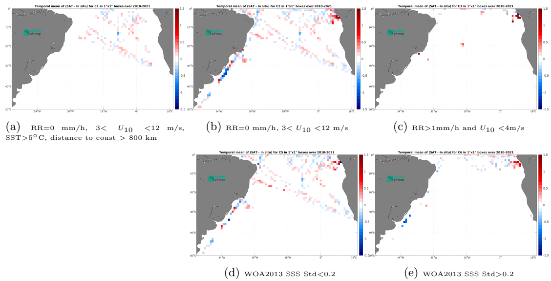
Figure 12: Temporal mean gridded over spatial boxes of size 1^\circ \times 1^\circ of \Delta\text{SSS} (SMOS SSS L3 v332 - 9 Days (CATDS-CPDC) - TSG (GOSUD-Research-vessel)) for 5 different subdatasets corresponding to:RR=0 mm/h, 3 < U_{10} < 12 m/s, SST>5°C, distance to coast > 800 km (a), RR=0 mm/h, 3 < U_{10} < 12 m/s (b), RR>1mm/h and U_{10} < 4 m/s (c), WOA2013 SSS Std<0.2 (d), WOA2013 SSS Std>0.2 (e).
