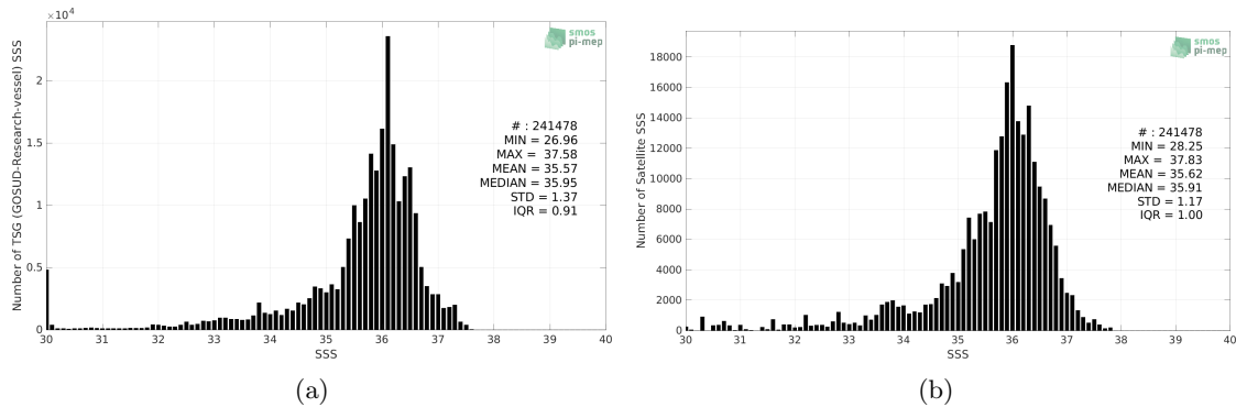
Figure 2: Histograms of SSS from TSG (GOSUD-Research-vessel) (a) and SMOS SSS L3 v332 - 9 Days (CATDS-CPDC) (b) considering all match-up pairs per bins of 0.1 over the South Atlantic Ocean Pi-MEP region and for the full satellite product period.
