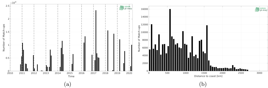
Figure 1: Number of match-ups between TSG (GOSUD-Research-vessel) and SMOS SSS L3 v332 - 9 Days (CATDS-CPDC) SSS as a function of time (a) and as function of the distance to coast (b) over the South Atlantic Ocean Pi-MEP region and for the full satellite product period.
