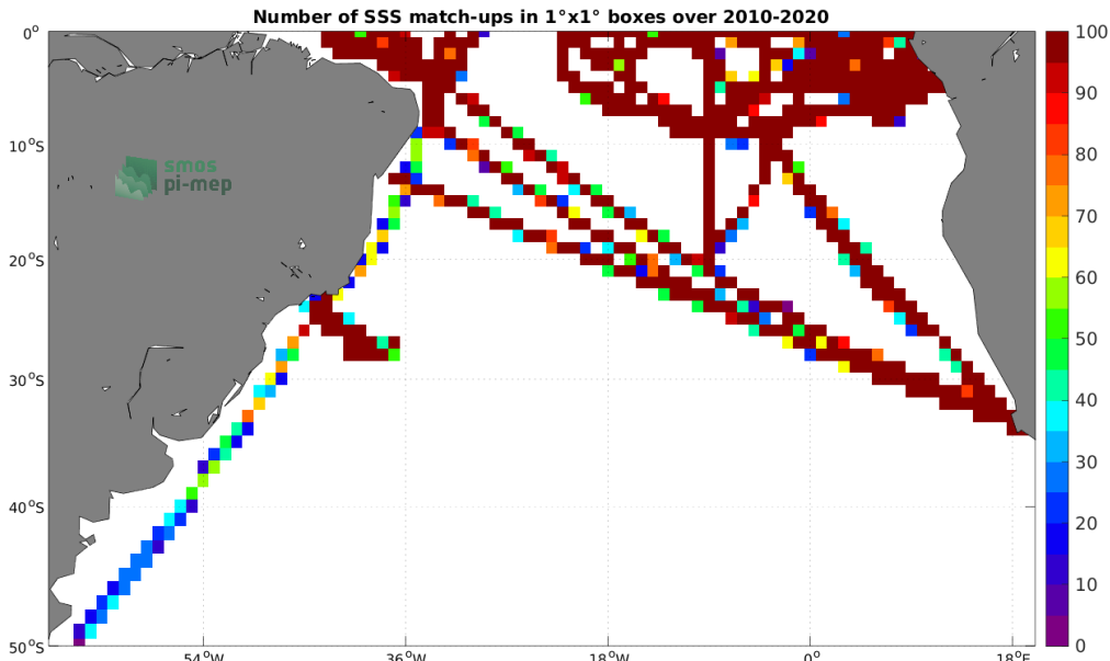
Figure 4: Number of SSS match-ups between TSG (GOSUD-Research-vessel) SSS and the SMOS SSS L3 v332 - 9 Days (CATDS-CPDC) SSS product for the South Atlantic Ocean Pi-MEP region over 1^\circ \times 1^\circ boxes and for the full satellite product period.
