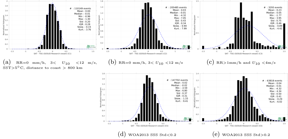
Figure 13: Normalized histogram of \Delta SSS (SMOS SSS L3 v332 - 9 Days (CATDS-CPDC) - TSG (GOSUD-Research-vessel)) for 5 different subdatasets corresponding to: RR=0 mm/h, 3 < U_{10} < 12 m/s, SST>5°C, distance to coast > 800 km (a), RR=0 mm/h, 3 < U_{10} < 12 m/s (b), RR>1mm/h and U_{10} < 4 m/s (c), WOA2013 SSS Std<0.2 (d), WOA2013 SSS Std>0.2 (e).
