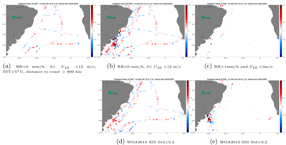
Figure 14: Temporal mean gridded over spatial boxes of size 1^\circ \times 1^\circ of \Delta\text{SSS} (SMOS SSS L3 v332 - 9 Days (CATDS-CPDC) - TSG (CSIC-UTM)) for 5 different subdatasets corresponding to:RR=0 mm/h, 3 < U_{10} < 12 m/s, SST >5^\circ\text{C} , distance to coast > 800 km (a), RR=0 mm/h, 3 < U_{10} < 12 m/s (b), RR >1 mm/h and U_{10} < 4 m/s (c), WOA2013 SSS Std <0.2 (d), WOA2013 SSS Std >0.2 (e).
