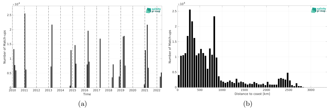
Figure 1: Number of match-ups between TSG (CSIC-UTM) and SMOS SSS L3 v332 - 9 Days (CATDS-CPDC) SSS as a function of time (a) and as function of the distance to coast (b) over the South Atlantic Ocean Pi-MEP region and for the full satellite product period.
