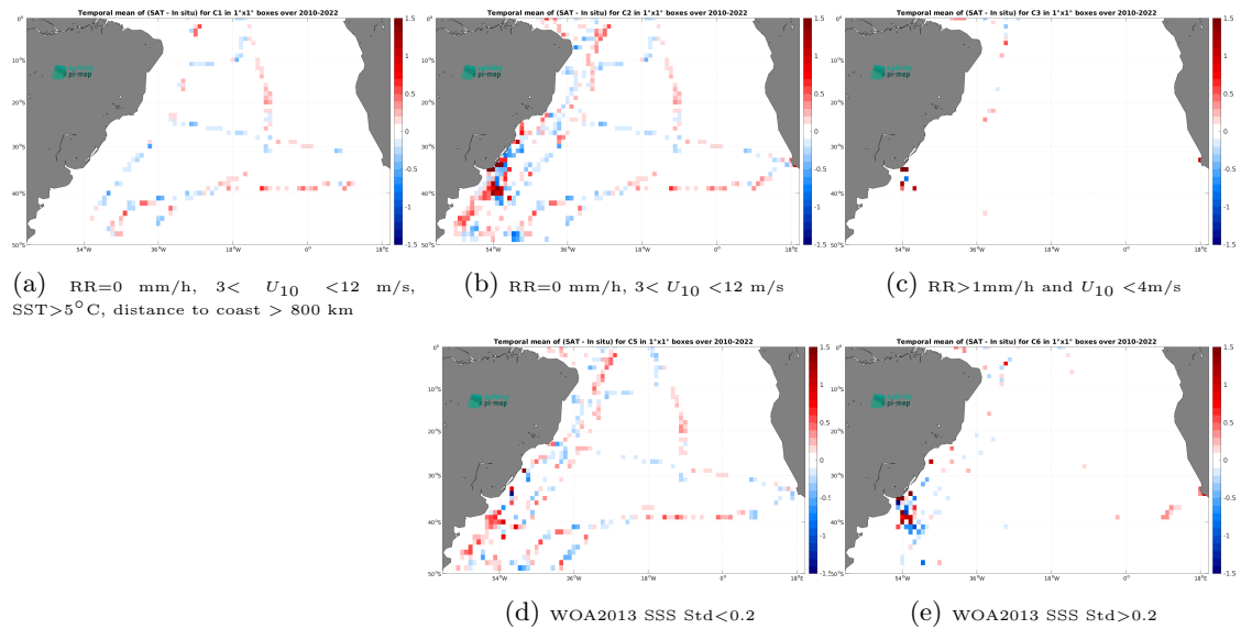
Figure 12: Temporal mean gridded over spatial boxes of size 1^\circ \times 1^\circ of \Delta\text{SSS} (SMOS SSS L3 v332 - 9 Days (CATDS-CPDC) - TSG (CSIC-UTM)) for 5 different subdatasets corresponding to:RR=0 mm/h, 3 < U_{10} < 12 m/s, SST >5^\circ\text{C} , distance to coast > 800 km (a), RR=0 mm/h, 3 < U_{10} < 12 m/s (b), RR >1 mm/h and U_{10} < 4 m/s (c), WOA2013 SSS Std <0.2 (d), WOA2013 SSS Std >0.2 (e).
