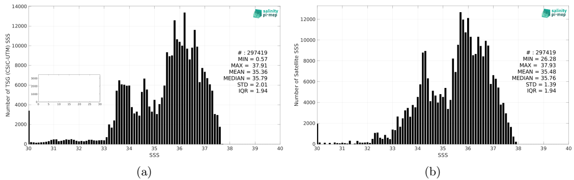
Figure 2: Histograms of SSS from TSG (CSIC-UTM) (a) and SMOS SSS L3 v332 - 9 Days (CATDS-CPDC) (b) considering all match-up pairs per bins of 0.1 over the South Atlantic Ocean Pi-MEP region and for the full satellite product period.
