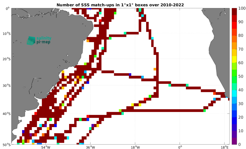
Figure 4: Number of SSS match-ups between TSG (CSIC-UTM) SSS and the SMOS SSS L3 v332 - 9 Days (CATDS-CPDC) SSS product for the South Atlantic Ocean Pi-MEP region over 1^\circ \times 1^\circ boxes and for the full satellite product period.
