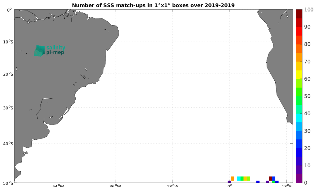
Figure 5: Number of SSS match-ups between Saildrone SSS and the SMOS SSS L3 v332 - 9 Days (CATDS-CPDC) SSS product for the South Atlantic Ocean Pi-MEP region over 1^\circ \times 1^\circ boxes and for the full satellite product period.
