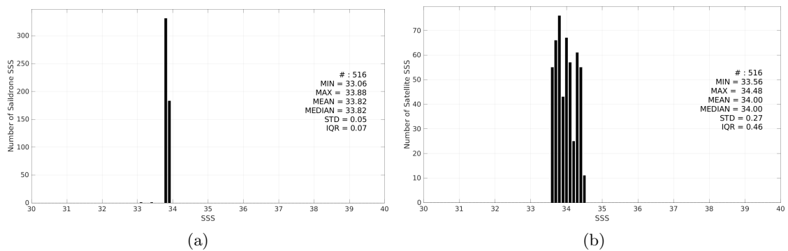
Figure 3: Histograms of SSS from Saildrone (a) and SMOS SSS L3 v332 - 9 Days (CATDS-CPDC) (b) considering all match-up pairs per bins of 0.1 over the South Atlantic Ocean Pi-MEP region and for the full satellite product period.
