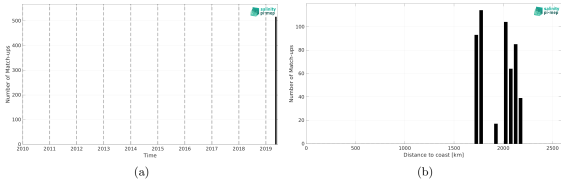
Figure 2: Number of match-ups between Saildrone and SMOS SSS L3 v332 - 9 Days (CATDS-CPDC) SSS as a function of time (a) and as function of the distance to coast (b) over the South Atlantic Ocean Pi-MEP region and for the full satellite product period.
