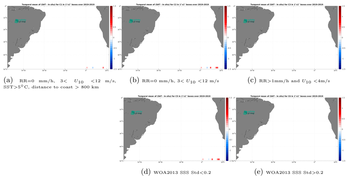
Figure 14: Temporal mean gridded over spatial boxes of size 1^\circ \times 1^\circ of \Delta SSS (SMOS SSS L3 v332 - 9 Days (CATDS-CPDC) - Saildrone) for 5 different subdatasets corresponding to:RR=0 mm/h, 3 < U_{10} < 12 m/s, SST>5°C, distance to coast > 800 km (a), RR=0 mm/h, 3 < U_{10} < 12 m/s (b), RR>1mm/h and U_{10} < 4 m/s (c), WOA2013 SSS Std<0.2 (d), WOA2013 SSS Std>0.2 (e).
