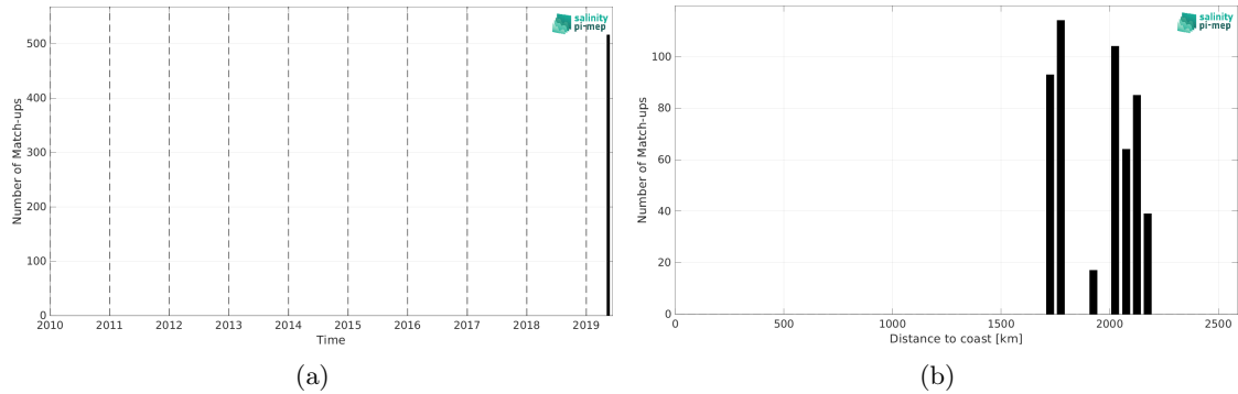
Figure 1: Number of match-ups between Saildrone and SMOS SSS L3 v332 - 9 Days (CATDS-CPDC) SSS as a function of time (a) and as function of the distance to coast (b) over the South Atlantic Ocean Pi-MEP region and for the full satellite product period.
