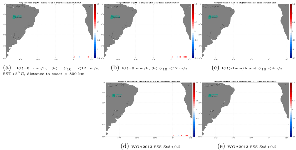
Figure 12: Temporal mean gridded over spatial boxes of size 1^{\circ}\times 1^{\circ} of \Delta\text{SSS} (SMOS SSS L3 v332 - 9 Days (CATDS-CPDC) - Sairdrone) for 5 different subdatasets corresponding to:RR=0 mm/h, 3 < U_{10} < 12 m/s, SST >5^{\circ}\text{C} , distance to coast > 800 km (a), RR=0 mm/h, 3 < U_{10} < 12 m/s (b), RR >1 mm/h and U_{10} < 4 m/s (c), WOA2013 SSS Std <0.2 (d), WOA2013 SSS Std >0.2 (e).
