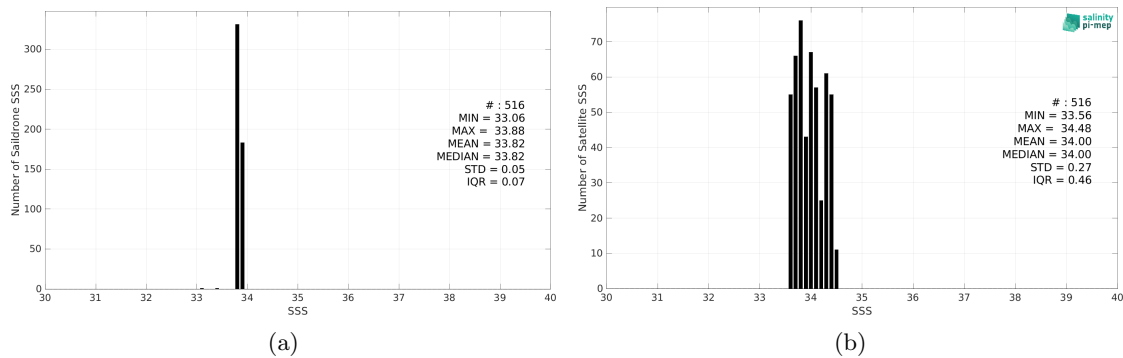
Figure 2: Histograms of SSS from Saildrone (a) and SMOS SSS L3 v332 - 9 Days (CATDS-CPDC) (b) considering all match-up pairs per bins of 0.1 over the South Atlantic Ocean Pi-MEP region and for the full satellite product period.
