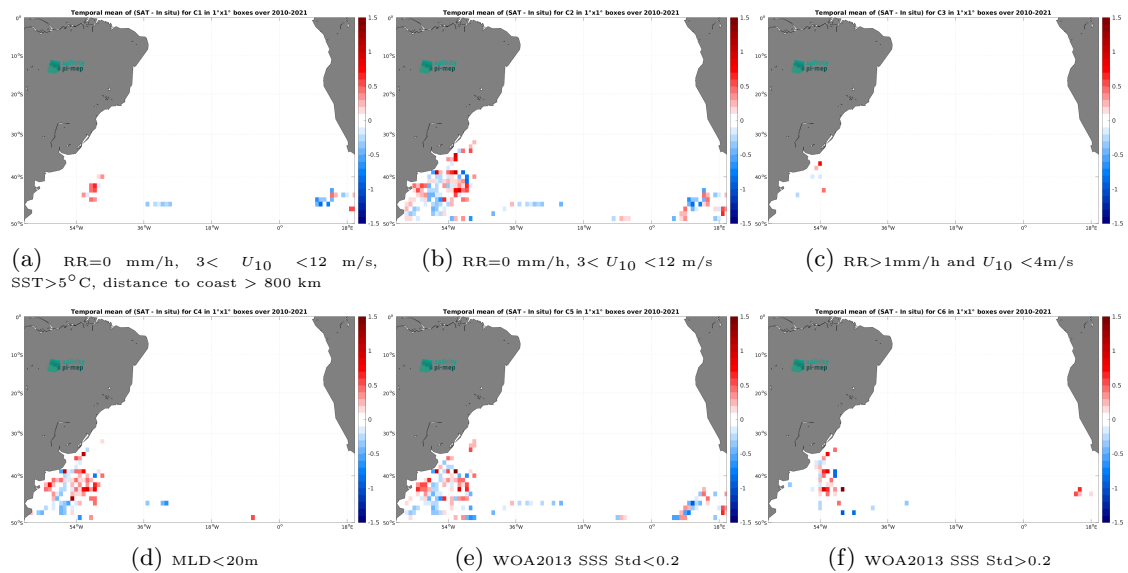
Figure 14: Temporal mean gridded over spatial boxes of size 1^\circ \times 1^\circ of \Delta SSS (SMOS SSS L3 v332 - 9 Days (CATDS-CPDC) - Marine mammals) for 6 different subdatasets corresponding to:RR=0 mm/h, 3 < U_{10} < 12 m/s, SST>5°C, distance to coast > 800 km (a), RR=0 mm/h, 3 < U_{10} < 12 m/s (b), RR>1mm/h and U_{10} < 4 m/s (c),MLD<20m (d),WOA2013 SSS Std<0.2 (e),WOA2013 SSS Std>0.2 (f).
