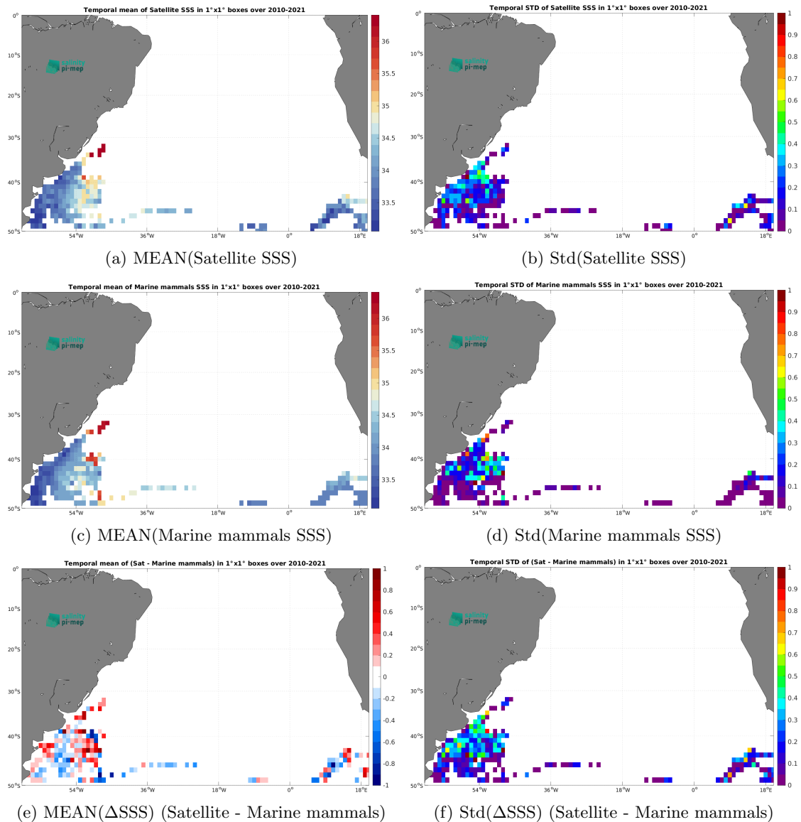
Figure 7: Temporal mean (left) and Std (right) of SSS from SMOS SSS L3 v332 - 9 Days (CATDS-CPDC) (top), Marine mammals (middle), and of \Delta SSS (Satellite - Marine mammals). Only match-up pairs are used to generate these maps.
