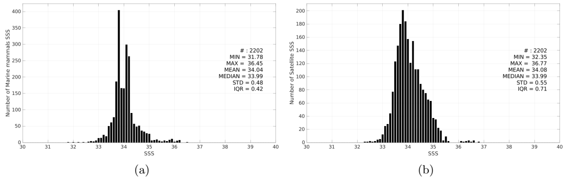
Figure 3: Histograms of SSS from Marine mammals (a) and SMOS SSS L3 v332 - 9 Days (CATDS-CPDC) (b) considering all match-up pairs per bins of 0.1 over the South Atlantic Ocean Pi-MEP region and for the full satellite product period.
