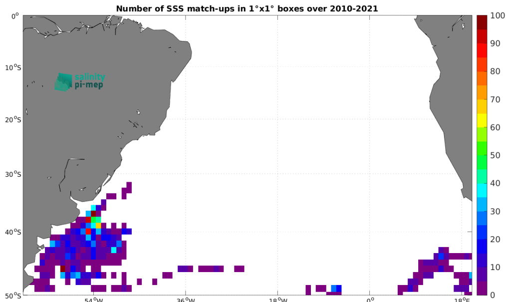
Figure 5: Number of SSS match-ups between Marine mammals SSS and the SMOS SSS L3 v332 - 9 Days (CATDS-CPDC) SSS product for the South Atlantic Ocean Pi-MEP region over 1^\circ \times 1^\circ boxes and for the full satellite product period.
