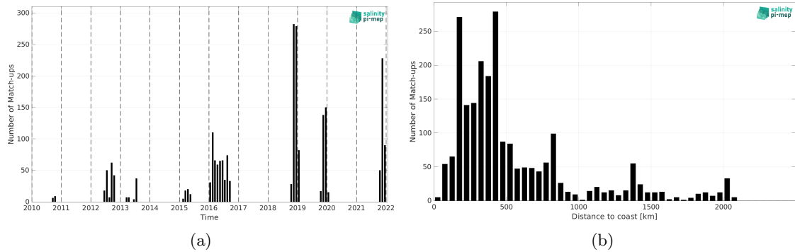
Figure 2: Number of match-ups between Marine mammals and SMOS SSS L3 v332 - 9 Days (CATDS-CPDC) SSS as a function of time (a) and as function of the distance to coast (b) over the South Atlantic Ocean Pi-MEP region and for the full satellite product period.
