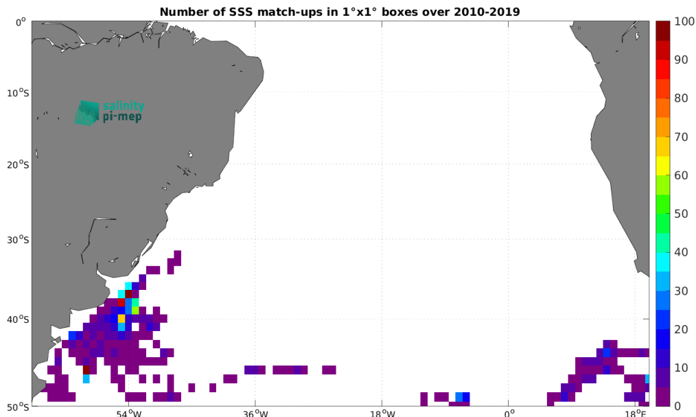
Figure 4: Number of SSS match-ups between Marine mammals SSS and the SMOS SSS L3 v332 - 9 Days (CATDS-CPDC) SSS product for the South Atlantic Ocean Pi-MEP region over 1^\circ \times 1^\circ boxes and for the full satellite product period.
