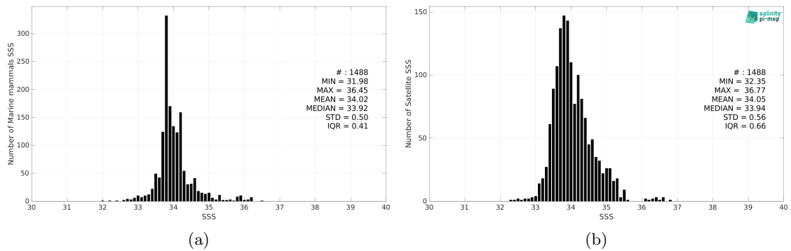
Figure 2: Histograms of SSS from Marine mammals (a) and SMOS SSS L3 v332 - 9 Days (CATDS-CPDC) (b) considering all match-up pairs per bins of 0.1 over the South Atlantic Ocean Pi-MEP region and for the full satellite product period.
