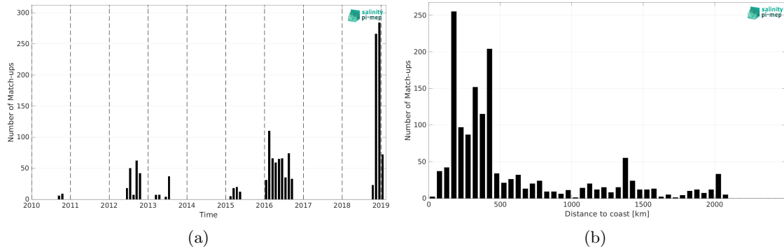
Figure 1: Number of match-ups between Marine mammals and SMOS SSS L3 v332 - 9 Days (CATDS-CPDC) SSS as a function of time (a) and as function of the distance to coast (b) over the South Atlantic Ocean Pi-MEP region and for the full satellite product period.
