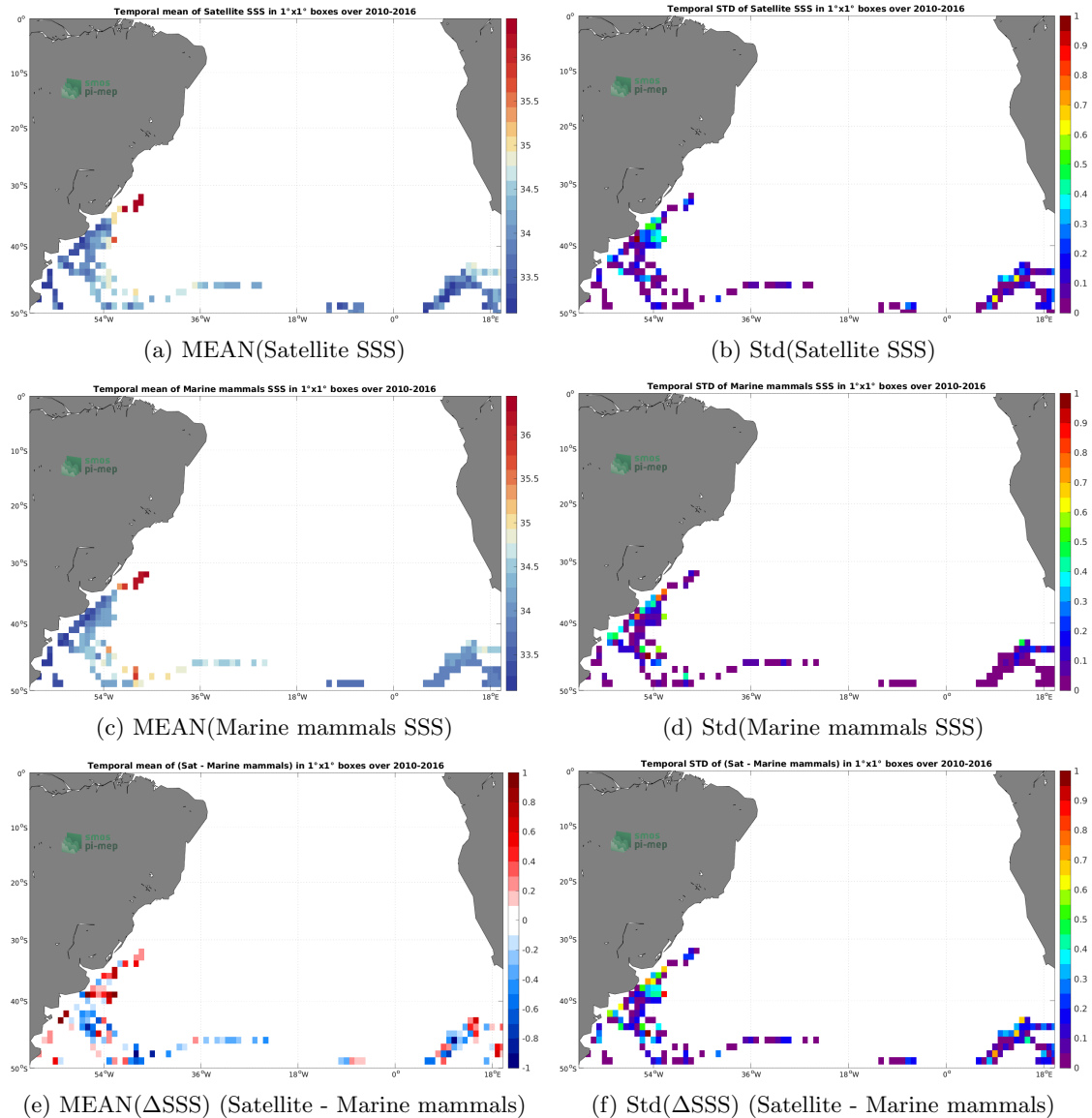
Figure 6: Temporal mean (left) and Std (right) of SSS from SMOS SSS L3 v332 - 9 Days (CATDS-CPDC) (top), Marine mammals (middle), and of \Delta SSS (Satellite - Marine mammals). Only match-up pairs are used to generate these maps.
