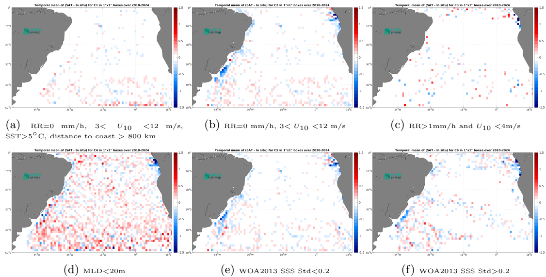
Figure 14: Temporal mean gridded over spatial boxes of size 1^\circ \times 1^\circ of \Delta\text{SSS} (SMOS SSS L3 v332 - 9 Days (CATDS-CPDC) - Argo) for 6 different subdatasets corresponding to: RR=0 mm/h, 3 < U_{10} < 12 m/s, SST>5°C, distance to coast > 800 km (a), RR=0 mm/h, 3 < U_{10} < 12 m/s (b), RR>1mm/h and U_{10} < 4 m/s (c),MLD<20m (d),WOA2013 SSS Std<0.2 (e),WOA2013 SSS Std>0.2 (f).
