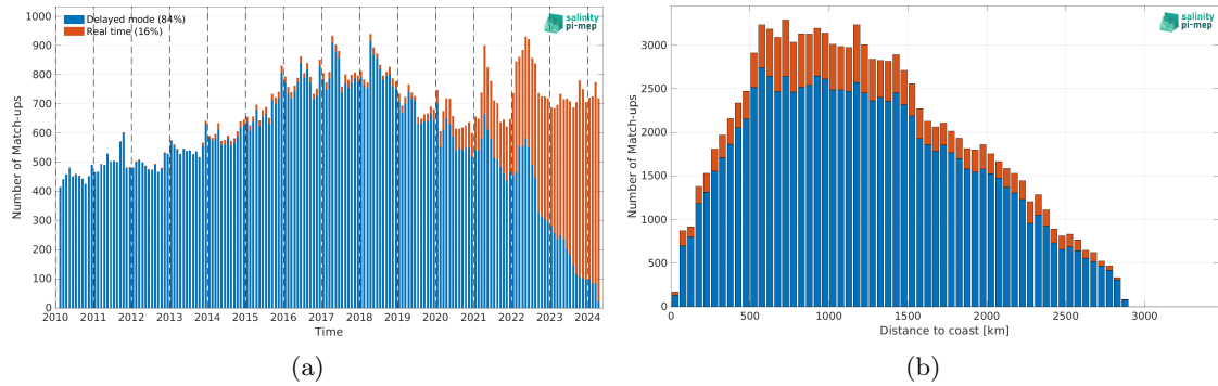
Figure 2: Number of match-ups between Argo and SMOS SSS L3 v332 - 9 Days (CATDS-CPDC) SSS as a function of time (a) and as function of the distance to coast (b) over the South Atlantic Ocean Pi-MEP region and for the full satellite product period.
