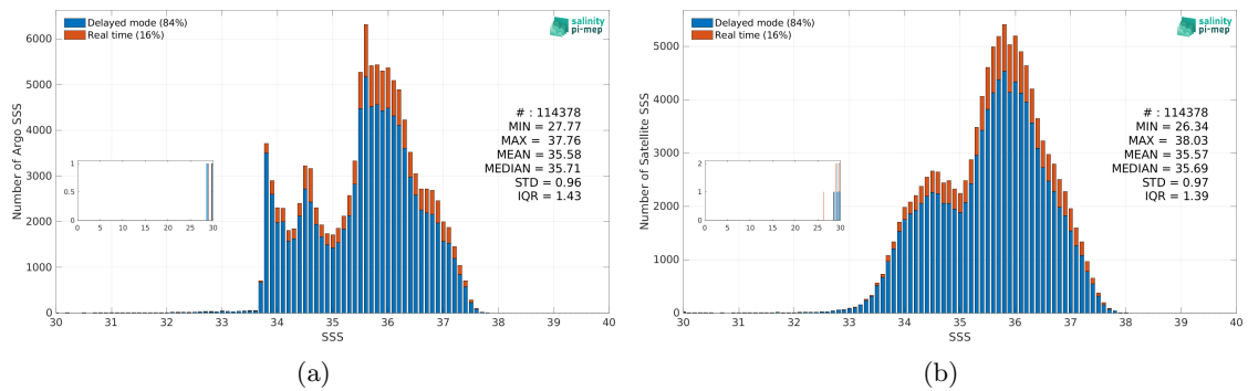
Figure 3: Histograms of SSS from Argo (a) and SMOS SSS L3 v332 - 9 Days (CATDS-CPDC) (b) considering all match-up pairs per bins of 0.1 over the South Atlantic Ocean Pi-MEP region and for the full satellite product period.
