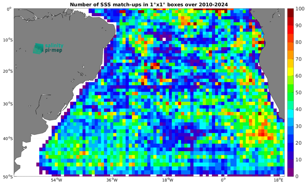
Figure 5: Number of SSS match-ups between Argo SSS and the SMOS SSS L3 v332 - 9 Days (CATDS-CPDC) SSS product for the South Atlantic Ocean Pi-MEP region over 1^\circ \times 1^\circ boxes and for the full satellite product period.
