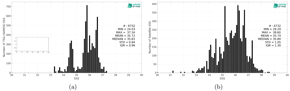
Figure 2: Histograms of SSS from TSG (SAMOS) (a) and SMOS SSS L2Q v331 - 0.25 Deg (CATDS-CPDC) (b) considering all match-up pairs per bins of 0.1 over the South Atlantic Ocean Pi-MEP region and for the full satellite product period.
