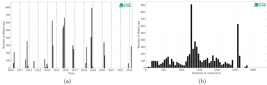
Figure 1: Number of match-ups between TSG (SAMOS) and SMOS SSS L2Q v331 - 0.25 Deg (CATDS-CPDC) SSS as a function of time (a) and as function of the distance to coast (b) over the South Atlantic Ocean Pi-MEP region and for the full satellite product period.
