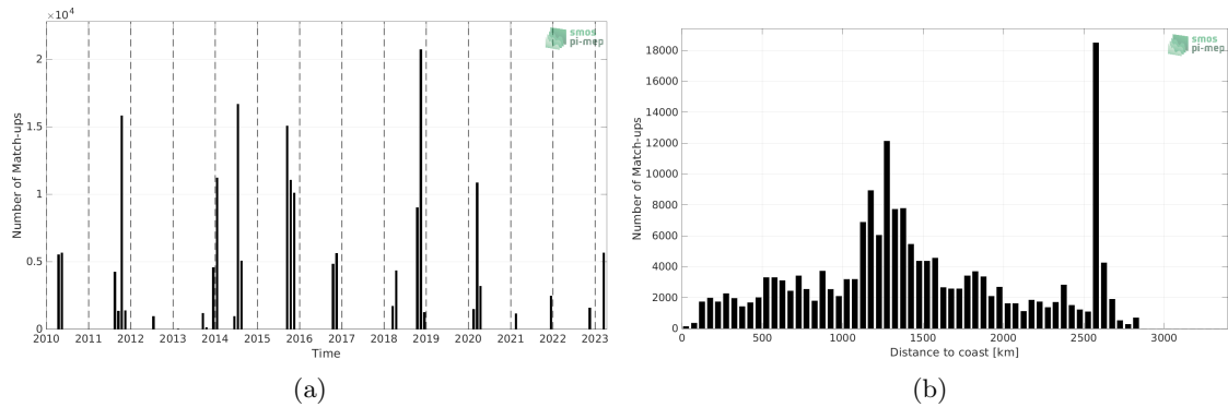
Figure 1: Number of match-ups between TSG (SAMOS) and SMOS SSS L2Q v331 - 0.25 Deg (CATDS-CPDC) SSS as a function of time (a) and as function of the distance to coast (b) over the South Atlantic Ocean Pi-MEP region and for the full satellite product period.
