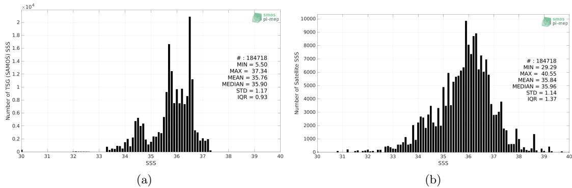
Figure 2: Histograms of SSS from TSG (SAMOS) (a) and SMOS SSS L2Q v331 - 0.25 Deg (CATDS-CPDC) (b) considering all match-up pairs per bins of 0.1 over the South Atlantic Ocean Pi-MEP region and for the full satellite product period.
