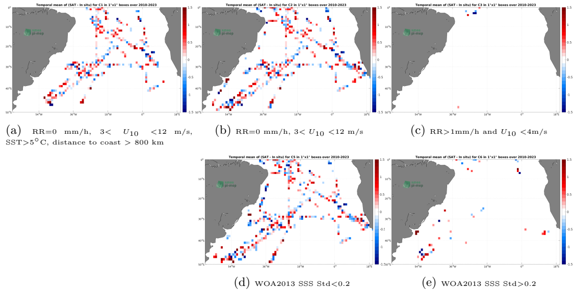
Figure 12: Temporal mean gridded over spatial boxes of size 1^\circ \times 1^\circ of \Delta\text{SSS} (SMOS SSS L2Q v331 - 0.25 Deg (CATDS-CPDC) - TSG (SAMOS)) for 5 different subdatasets corresponding to:RR=0 mm/h, 3 < U_{10} < 12 m/s, SST >5^\circ\text{C} , distance to coast > 800 km (a), RR=0 mm/h, 3 < U_{10} < 12 m/s (b), RR >1 mm/h and U_{10} < 4 m/s (c), WOA2013 SSS Std <0.2 (d), WOA2013 SSS Std >0.2 (e).
