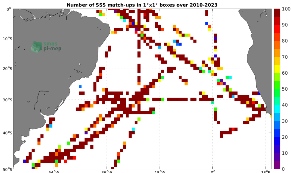
Figure 4: Number of SSS match-ups between TSG (SAMOS) SSS and the SMOS SSS L2Q v331 - 0.25 Deg (CATDS-CPDC) SSS product for the South Atlantic Ocean Pi-MEP region over 1^\circ \times 1^\circ boxes and for the full satellite product period.
