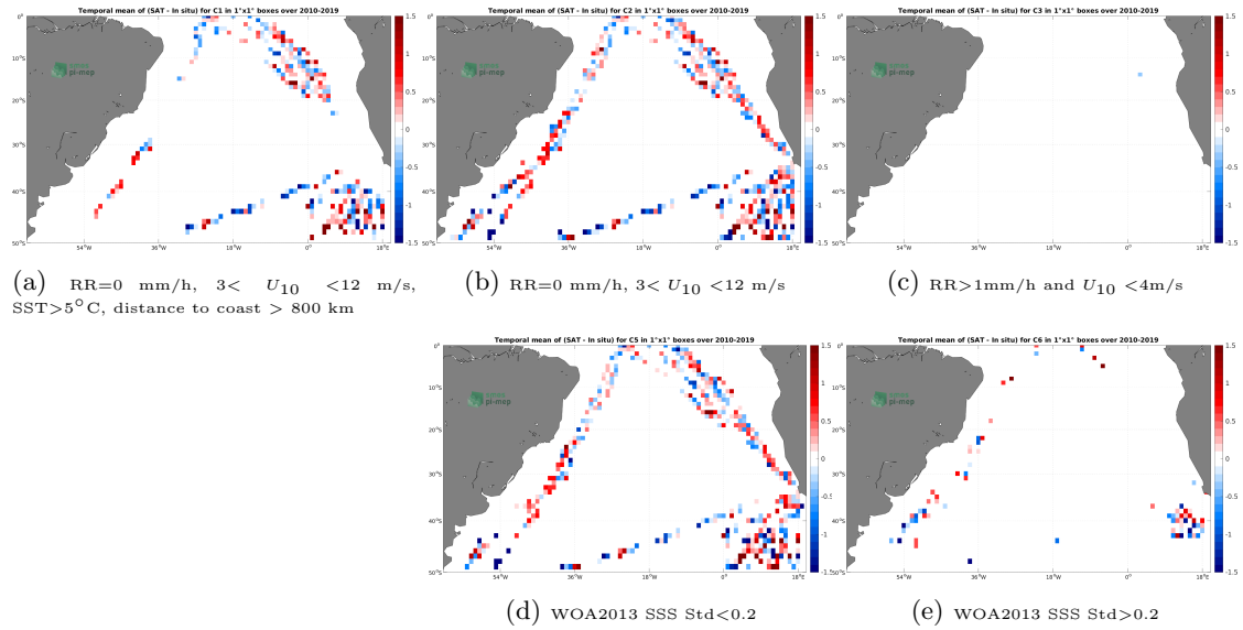
Figure 12: Temporal mean gridded over spatial boxes of size 1^\circ \times 1^\circ of \Delta SSS (SMOS SSS L2Q v331 - 0.25 Deg (CATDS-CPDC) - TSG (Polarstern)) for 5 different subdatasets corresponding to:RR=0 mm/h, 3 < U_{10} < 12 m/s, SST >5^\circ\text{C} , distance to coast > 800 km (a), RR=0 mm/h, 3 < U_{10} < 12 m/s (b), RR >1 mm/h and U_{10} < 4 m/s (c), WOA2013 SSS Std <0.2 (d), WOA2013 SSS Std >0.2 (e).
