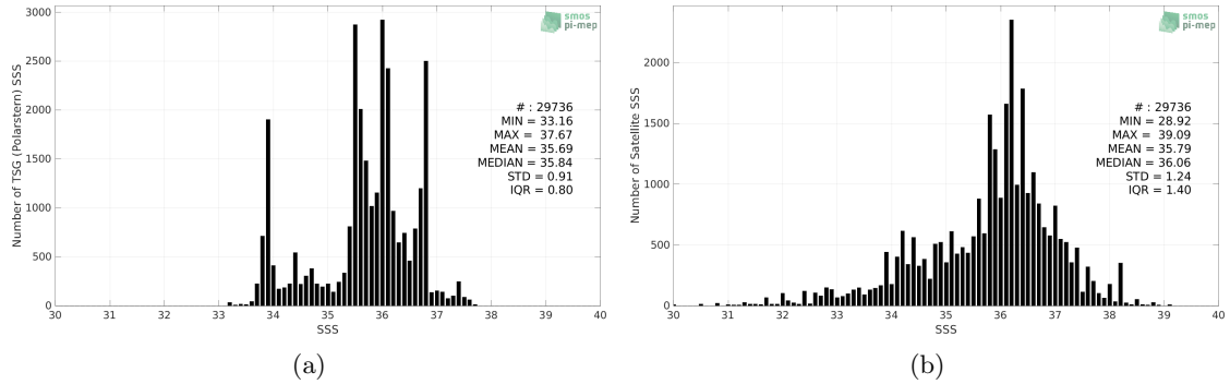
Figure 2: Histograms of SSS from TSG (Polarstern) (a) and SMOS SSS L2Q v331 - 0.25 Deg (CATDS-CPDC) (b) considering all match-up pairs per bins of 0.1 over the South Atlantic Ocean Pi-MEP region and for the full satellite product period.
