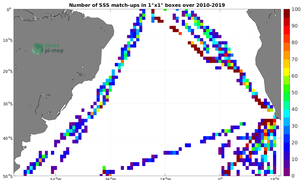
Figure 4: Number of SSS match-ups between TSG (Polarstern) SSS and the SMOS SSS L2Q v331 - 0.25 Deg (CATDS-CPDC) SSS product for the South Atlantic Ocean Pi-MEP region over 1^\circ \times 1^\circ boxes and for the full satellite product period.
