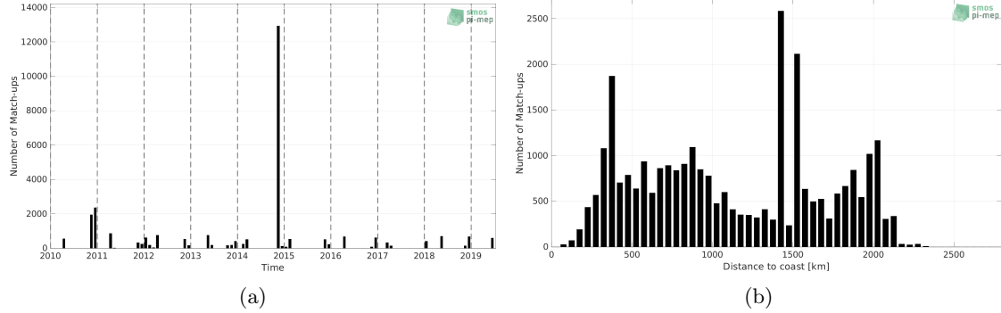
Figure 1: Number of match-ups between TSG (Polarstern) and SMOS SSS L2Q v331 - 0.25 Deg (CATDS-CPDC) SSS as a function of time (a) and as function of the distance to coast (b) over the South Atlantic Ocean Pi-MEP region and for the full satellite product period.
