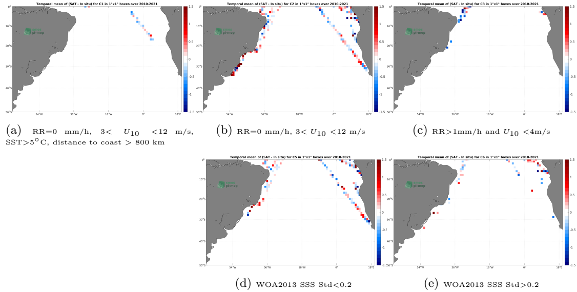
Figure 12: Temporal mean gridded over spatial boxes of size 1^{\circ}\times 1^{\circ} of \Delta\text{SSS} (SMOS SSS L2Q v331 - 0.25 Deg (CATDS-CPDC) - TSG (LEGOS-DM)) for 5 different subdatasets corresponding to:RR=0 mm/h, 3 < U_{10} < 12 m/s, SST >5^{\circ}\text{C} , distance to coast > 800 km (a), RR=0 mm/h, 3 < U_{10} < 12 m/s (b), RR >1 mm/h and U_{10} < 4 m/s (c), WOA2013 SSS Std <0.2 (d), WOA2013 SSS Std >0.2 (e).
