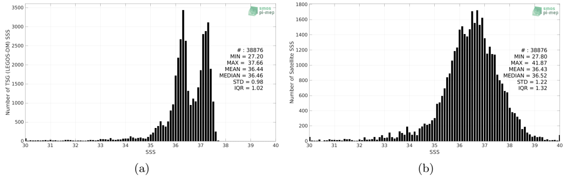
Figure 2: Histograms of SSS from TSG (LEGOS-DM) (a) and SMOS SSS L2Q v331 - 0.25 Deg (CATDS-CPDC) (b) considering all match-up pairs per bins of 0.1 over the South Atlantic Ocean Pi-MEP region and for the full satellite product period.
