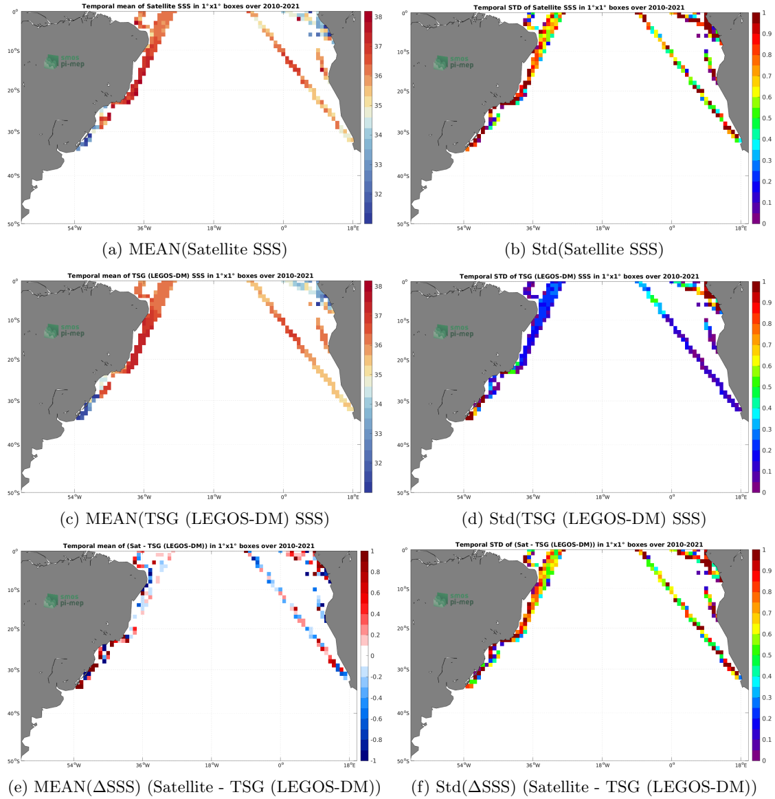
Figure 6: Temporal mean (left) and Std (right) of SSS from SMOS SSS L2Q v331 - 0.25 Deg (CATDS-CPDC) (top), TSG (LEGOS-DM) (middle), and of \Delta SSS (Satellite - TSG (LEGOS-DM)). Only match-up pairs are used to generate these maps.
