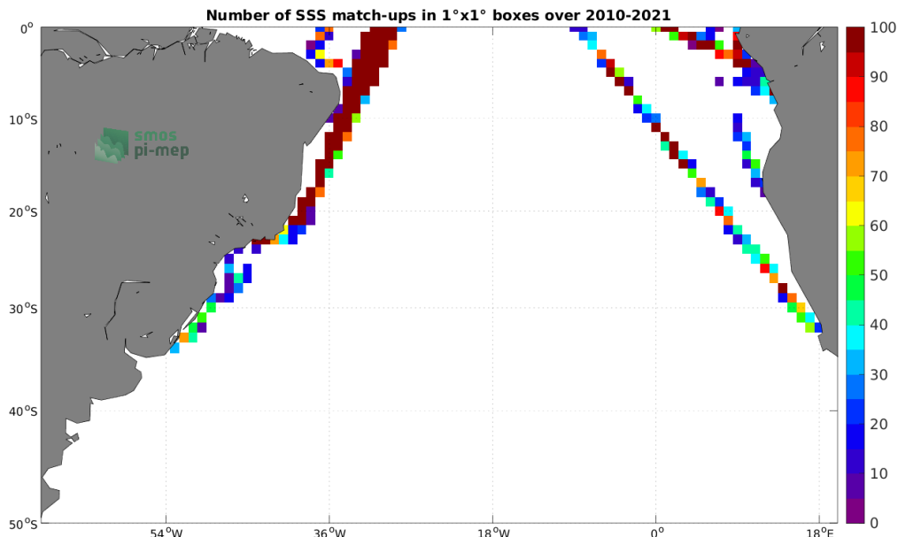
Figure 4: Number of SSS match-ups between TSG (LEGOS-DM) SSS and the SMOS SSS L2Q v331 - 0.25 Deg (CATDS-CPDC) SSS product for the South Atlantic Ocean Pi-MEP region over 1^\circ \times 1^\circ boxes and for the full satellite product period.
