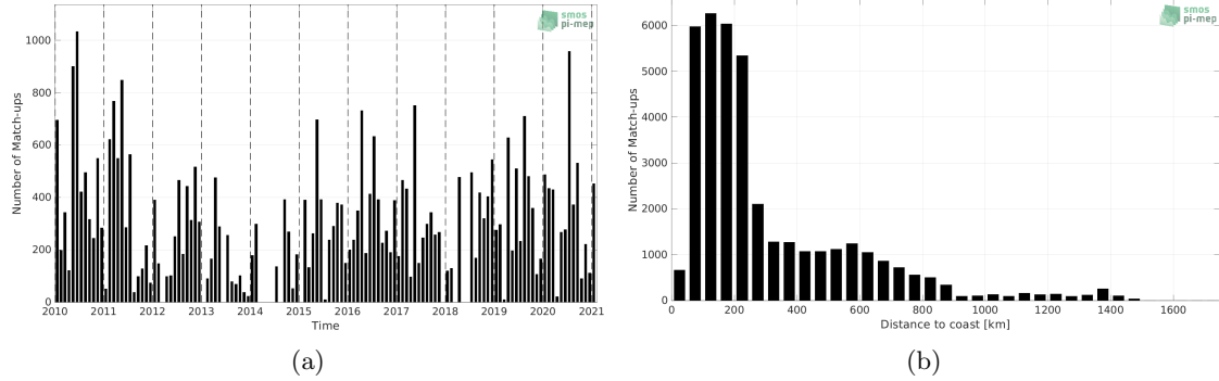
Figure 1: Number of match-ups between TSG (LEGOS-DM) and SMOS SSS L2Q v331 - 0.25 Deg (CATDS-CPDC) SSS as a function of time (a) and as function of the distance to coast (b) over the South Atlantic Ocean Pi-MEP region and for the full satellite product period.
