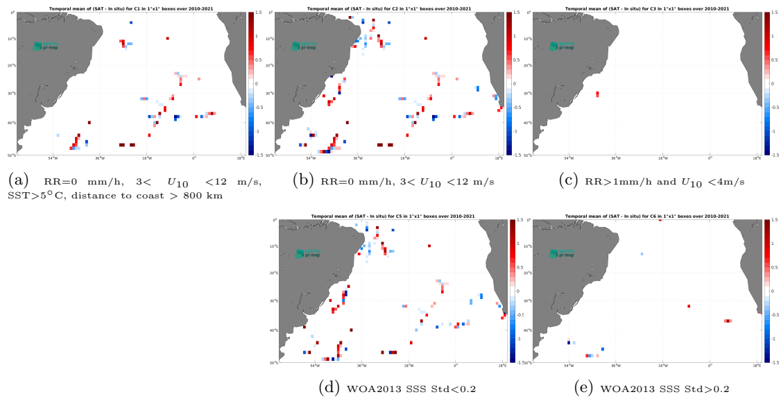
Figure 12: Temporal mean gridded over spatial boxes of size 1^\circ \times 1^\circ of \Delta\text{SSS} (SMOS SSS L2Q v331 - 0.25 Deg (CATDS-CPDC) - TSG (GOSUD-Sailing-ship)) for 5 different subdatasets corresponding to:RR=0 mm/h, 3 < U_{10} < 12 m/s, SST >5^\circ\text{C} , distance to coast > 800 km (a), RR=0 mm/h, 3 < U_{10} < 12 m/s (b), RR >1 mm/h and U_{10} < 4 m/s (c), WOA2013 SSS Std <0.2 (d), WOA2013 SSS Std >0.2 (e).
