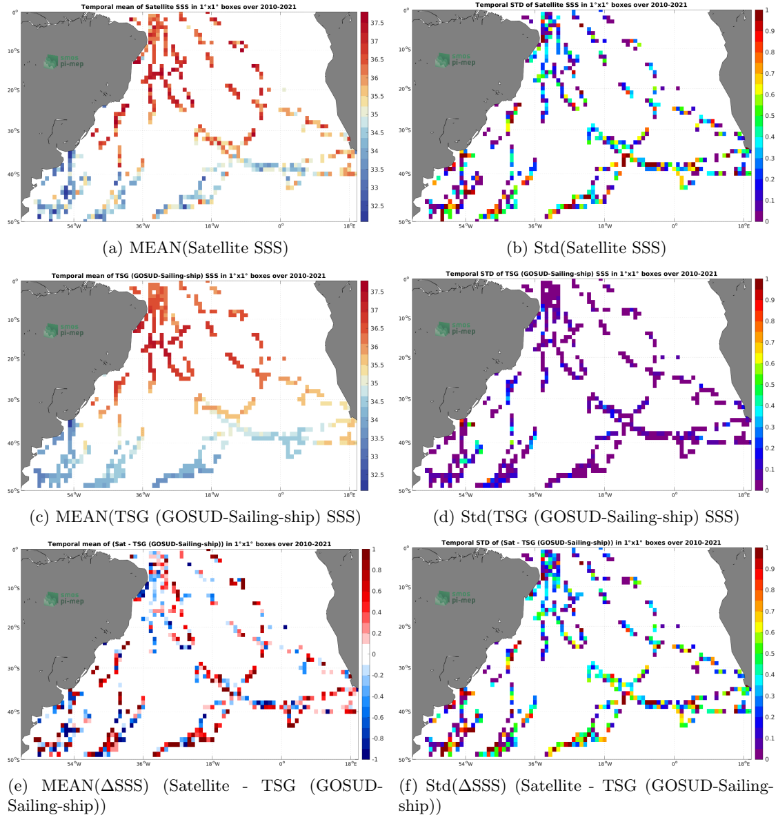
Figure 6: Temporal mean (left) and Std (right) of SSS from SMOS SSS L2Q v331 - 0.25 Deg (CATDS-CPDC) (top), TSG (GOSUD-Sailing-ship) (middle), and of \Delta SSS (Satellite - TSG (GOSUD-Sailing-ship)). Only match-up pairs are used to generate these maps.
