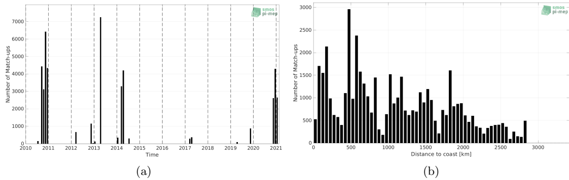
Figure 1: Number of match-ups between TSG (GOSUD-Sailing-ship) and SMOS SSS L2Q v331 - 0.25 Deg (CATDS-CPDC) SSS as a function of time (a) and as function of the distance to coast (b) over the South Atlantic Ocean Pi-MEP region and for the full satellite product period.
