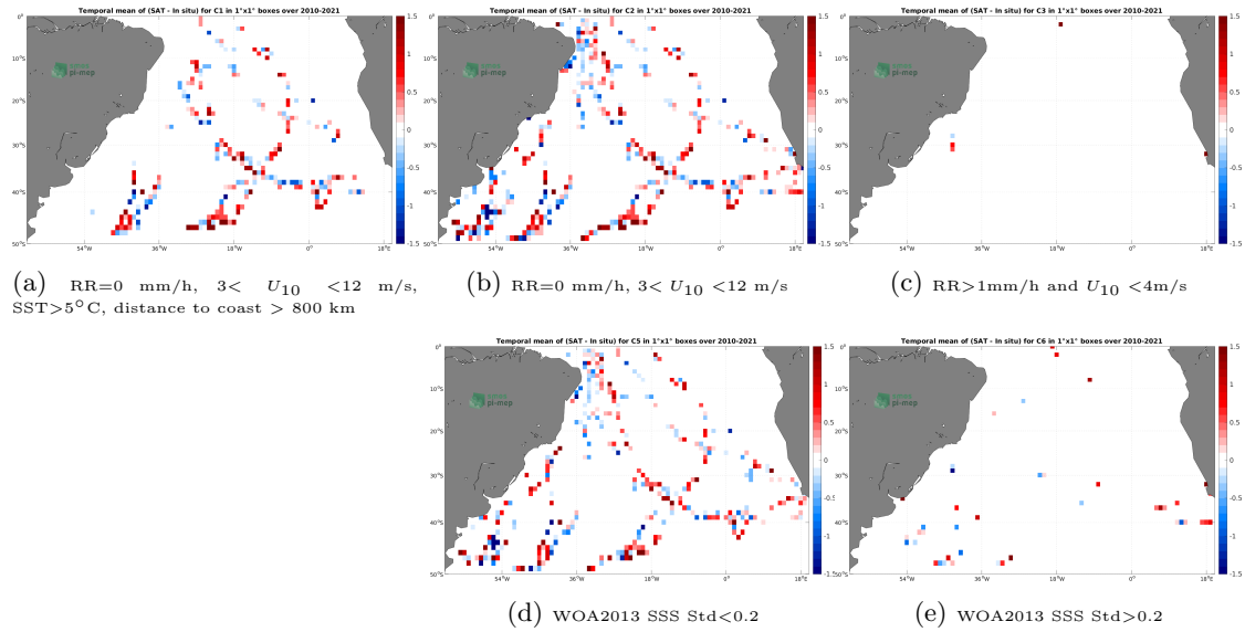
Figure 12: Temporal mean gridded over spatial boxes of size 1^\circ \times 1^\circ of \Delta\text{SSS} (SMOS SSS L2Q v331 - 0.25 Deg (CATDS-CPDC) - TSG (GOSUD-Sailing-ship)) for 5 different subdatasets corresponding to:RR=0 mm/h, 3 < U_{10} < 12 m/s, SST >5^\circ\text{C} , distance to coast > 800 km (a), RR=0 mm/h, 3 < U_{10} < 12 m/s (b), RR >1 mm/h and U_{10} < 4 m/s (c), WOA2013 SSS Std <0.2 (d), WOA2013 SSS Std >0.2 (e).
