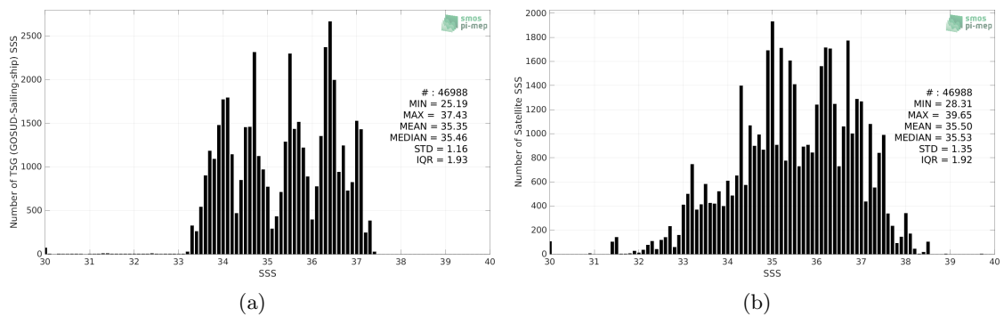
Figure 2: Histograms of SSS from TSG (GOSUD-Sailing-ship) (a) and SMOS SSS L2Q v331 - 0.25 Deg (CATDS-CPDC) (b) considering all match-up pairs per bins of 0.1 over the South Atlantic Ocean Pi-MEP region and for the full satellite product period.
