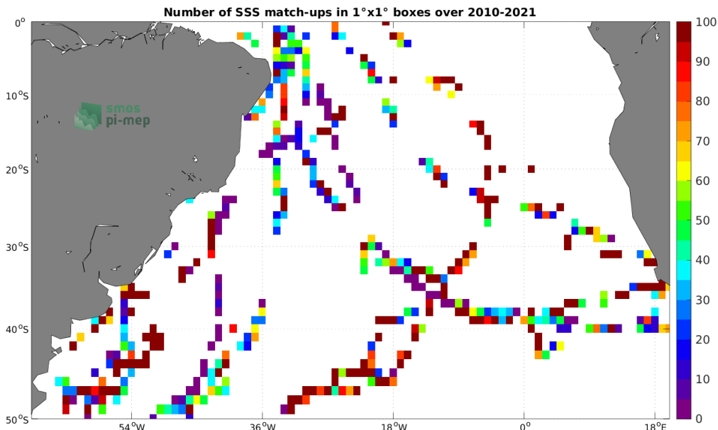
Figure 4: Number of SSS match-ups between TSG (GOSUD-Sailing-ship) SSS and the SMOS SSS L2Q v331 - 0.25 Deg (CATDS-CPDC) SSS product for the South Atlantic Ocean Pi-MEP region over 1^\circ \times 1^\circ boxes and for the full satellite product period.
