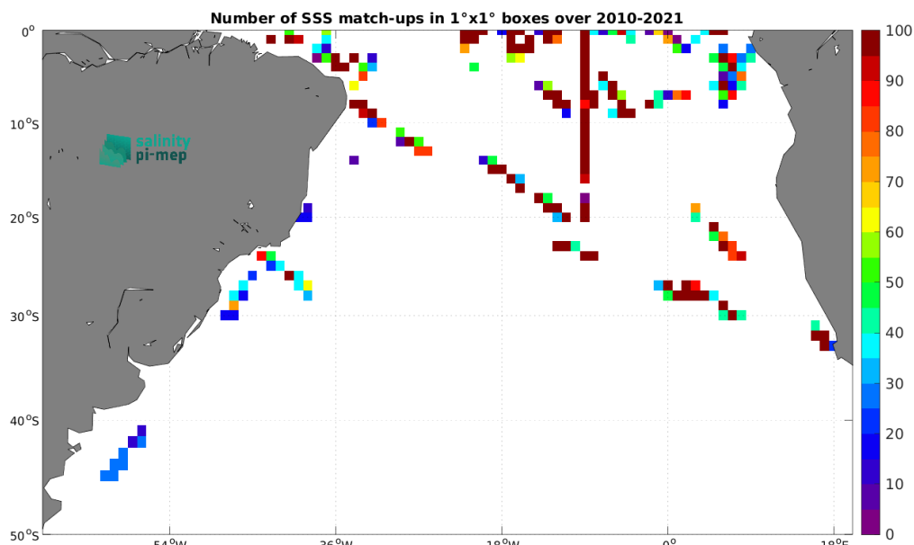
Figure 4: Number of SSS match-ups between TSG (GOSUD-Research-vessel) SSS and the SMOS SSS L2Q v331 - 0.25 Deg (CATDS-CPDC) SSS product for the South Atlantic Ocean Pi-MEP region over 1^\circ \times 1^\circ boxes and for the full satellite product period.
