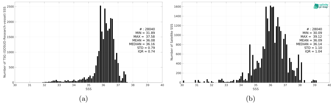
Figure 2: Histograms of SSS from TSG (GOSUD-Research-vessel) (a) and SMOS SSS L2Q v331 - 0.25 Deg (CATDS-CPDC) (b) considering all match-up pairs per bins of 0.1 over the South Atlantic Ocean Pi-MEP region and for the full satellite product period.
