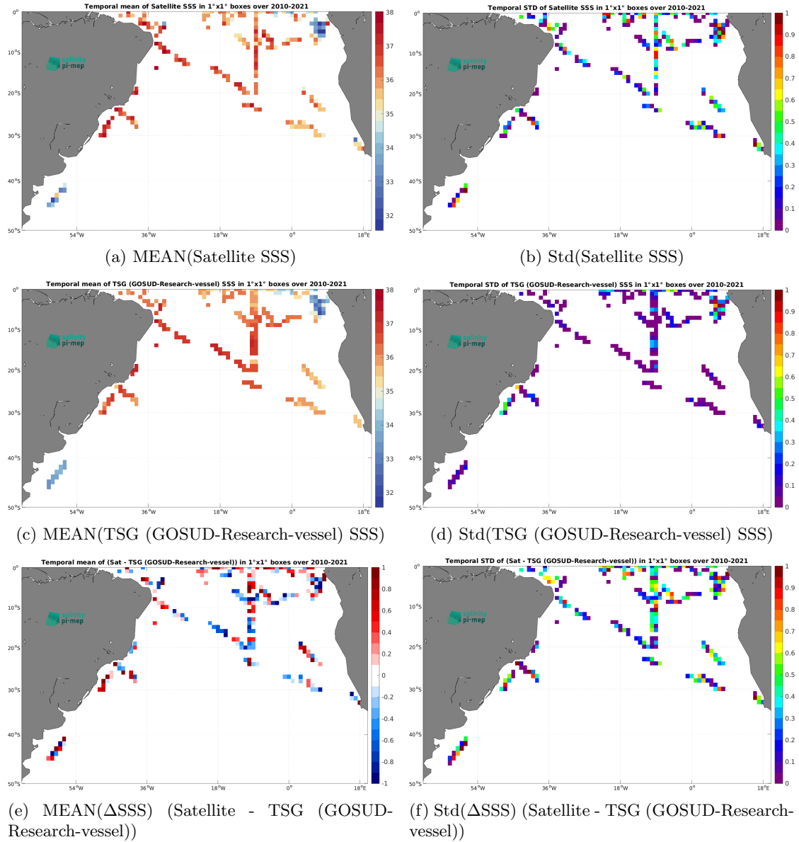
Figure 6: Temporal mean (left) and Std (right) of SSS from SMOS SSS L2Q v331 - 0.25 Deg (CATDS-CPDC) (top), TSG (GOSUD-Research-vessel) (middle), and of \Delta SSS (Satellite - TSG (GOSUD-Research-vessel)). Only match-up pairs are used to generate these maps.
