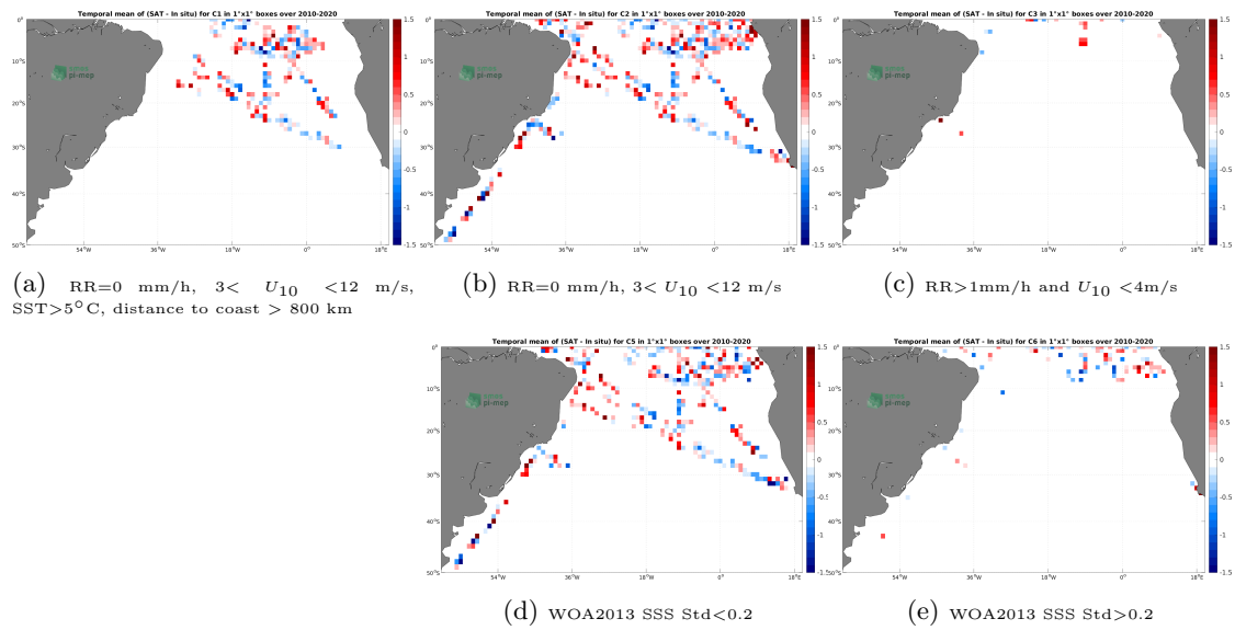
Figure 12: Temporal mean gridded over spatial boxes of size 1^\circ \times 1^\circ of \Delta\text{SSS} (SMOS SSS L2Q v331 - 0.25 Deg (CATDS-CPDC) - TSG (GOSUD-Research-vessel)) for 5 different subdatasets corresponding to:RR=0 mm/h, 3 < U_{10} < 12 m/s, SST>5°C, distance to coast > 800 km (a), RR=0 mm/h, 3 < U_{10} < 12 m/s (b), RR>1mm/h and U_{10} < 4 m/s (c), WOA2013 SSS Std<0.2 (d), WOA2013 SSS Std>0.2 (e).
