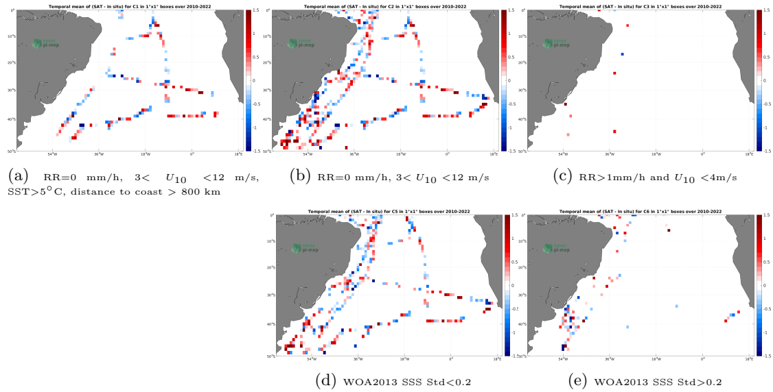
Figure 12: Temporal mean gridded over spatial boxes of size 1^\circ \times 1^\circ of \Delta\text{SSS} (SMOS SSS L2Q v331 - 0.25 Deg (CATDS-CPDC) - TSG (CSIC-UTM)) for 5 different subdatasets corresponding to:RR=0 mm/h, 3 < U_{10} < 12 m/s, SST >5^\circ\text{C} , distance to coast > 800 km (a), RR=0 mm/h, 3 < U_{10} < 12 m/s (b), RR >1 mm/h and U_{10} < 4 m/s (c), WOA2013 SSS Std <0.2 (d), WOA2013 SSS Std >0.2 (e).
