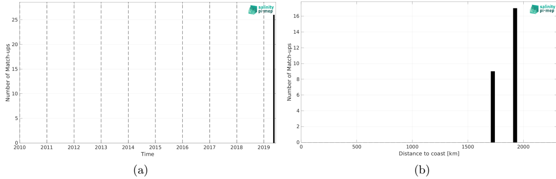
Figure 1: Number of match-ups between Saildrone and SMOS SSS L2Q v331 - 0.25 Deg (CATDS-CPDC) SSS as a function of time (a) and as function of the distance to coast (b) over the South Atlantic Ocean Pi-MEP region and for the full satellite product period.
