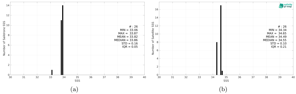
Figure 2: Histograms of SSS from Saildrone (a) and SMOS SSS L2Q v331 - 0.25 Deg (CATDS-CPDC) (b) considering all match-up pairs per bins of 0.1 over the South Atlantic Ocean Pi-MEP region and for the full satellite product period.
