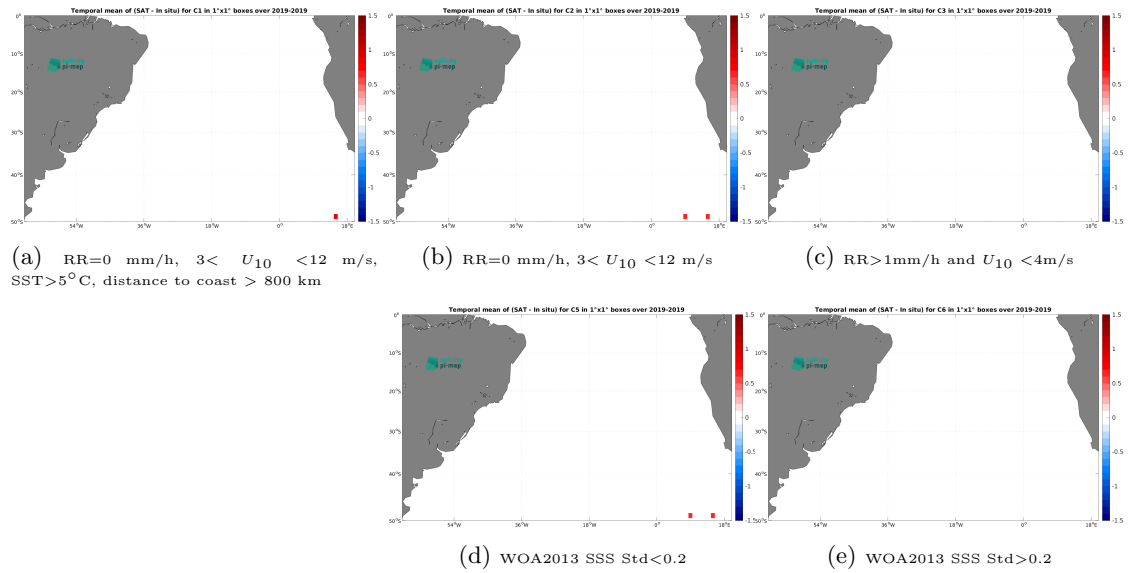
Figure 12: Temporal mean gridded over spatial boxes of size 1^{\circ}\times 1^{\circ} of \Delta\text{SSS} (SMOS SSS L2Q v331 - 0.25 Deg (CATDS-CPDC) - Saildrone) for 5 different subdatasets corresponding to:RR=0 mm/h, 3 < U_{10} < 12 m/s, SST >5^{\circ}\text{C} , distance to coast > 800 km (a), RR=0 mm/h, 3 < U_{10} < 12 m/s (b), RR >1 mm/h and U_{10} < 4 m/s (c), WOA2013 SSS Std <0.2 (d), WOA2013 SSS Std >0.2 (e).
