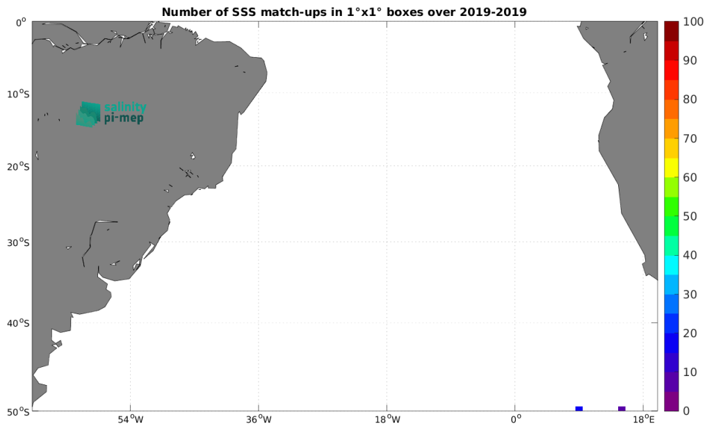
Figure 4: Number of SSS match-ups between Saildrone SSS and the SMOS SSS L2Q v331 - 0.25 Deg (CATDS-CPDC) SSS product for the South Atlantic Ocean Pi-MEP region over 1^\circ \times 1^\circ boxes and for the full satellite product period.
