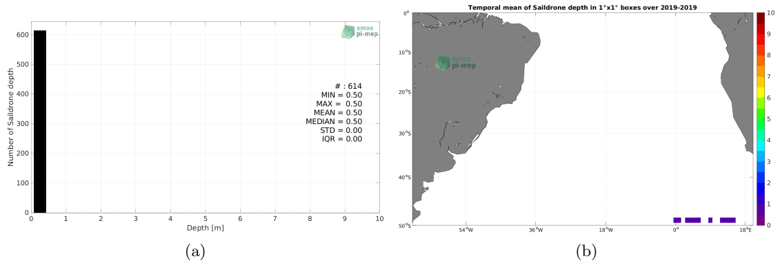
Figure 3: Histograms of the depth of the upper level SSS measurements from Sairdrone in the Match-up DataBase for the South Atlantic Ocean Pi-MEP region (a) and temporal mean spatial distribution of pressure of the in situ SSS data over 1^\circ \times 1^\circ boxes and for the full satellite product period (b).
