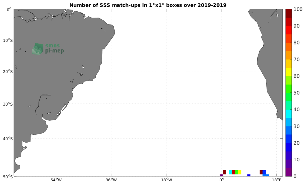
Figure 4: Number of SSS match-ups between Sairdrone SSS and the SMOS SSS L2Q v331 - 0.25 Deg (CATDS-CPDC) SSS product for the South Atlantic Ocean Pi-MEP region over 1^\circ \times 1^\circ boxes and for the full satellite product period.
