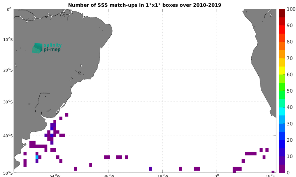
Figure 4: Number of SSS match-ups between Marine mammals SSS and the SMOS SSS L2Q v331 - 0.25 Deg (CATDS-CPDC) SSS product for the South Atlantic Ocean Pi-MEP region over 1^\circ \times 1^\circ boxes and for the full satellite product period.
