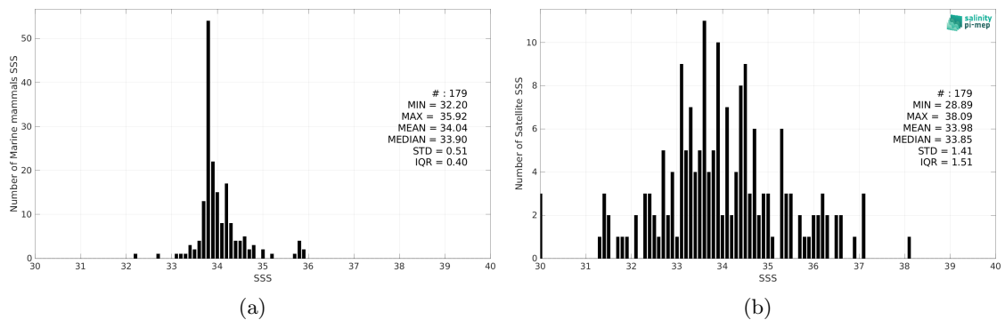
Figure 2: Histograms of SSS from Marine mammals (a) and SMOS SSS L2Q v331 - 0.25 Deg (CATDS-CPDC) (b) considering all match-up pairs per bins of 0.1 over the South Atlantic Ocean Pi-MEP region and for the full satellite product period.
