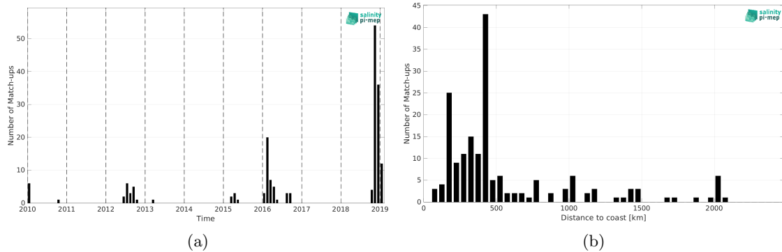
Figure 1: Number of match-ups between Marine mammals and SMOS SSS L2Q v331 - 0.25 Deg (CATDS-CPDC) SSS as a function of time (a) and as function of the distance to coast (b) over the South Atlantic Ocean Pi-MEP region and for the full satellite product period.
