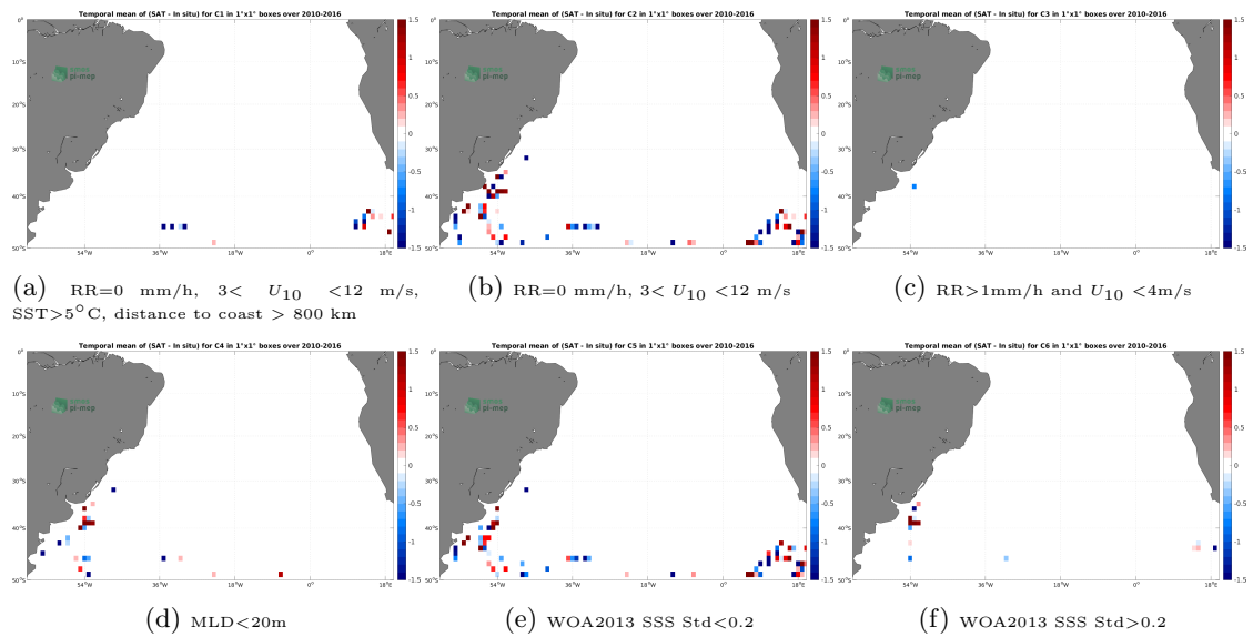
Figure 12: Temporal mean gridded over spatial boxes of size 1^\circ \times 1^\circ of \Delta SSS (SMOS SSS L2Q v331 - 0.25 Deg (CATDS-CPDC) - Marine mammals) for 6 different subdatasets corresponding to:RR=0 mm/h, 3 < U_{10} < 12 m/s, SST > 5^\circ\text{C} , distance to coast > 800 km (a), RR=0 mm/h, 3 < U_{10} < 12 m/s (b), RR > 1 mm/h and U_{10} < 4 m/s (c),MLD < 20 m (d),WOA2013 SSS Std < 0.2 (e),WOA2013 SSS Std > 0.2 (f).
