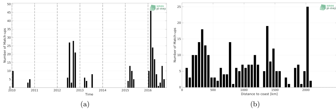
Figure 1: Number of match-ups between Marine mammals and SMOS SSS L2Q v331 - 0.25 Deg (CATDS-CPDC) SSS as a function of time (a) and as function of the distance to coast (b) over the South Atlantic Ocean Pi-MEP region and for the full satellite product period.
