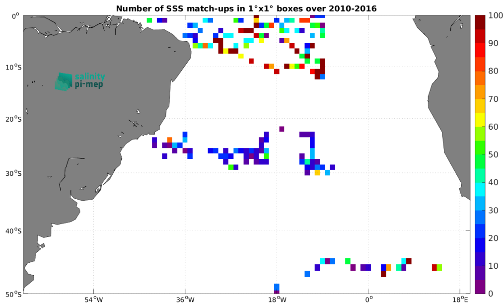
Figure 3: Number of SSS match-ups between Surface drifters SSS and the SMOS SSS L2Q v331 - 0.25 Deg (CATDS-CPDC) SSS product for the South Atlantic Ocean Pi-MEP region over 1^\circ \times 1^\circ boxes and for the full satellite product period.
