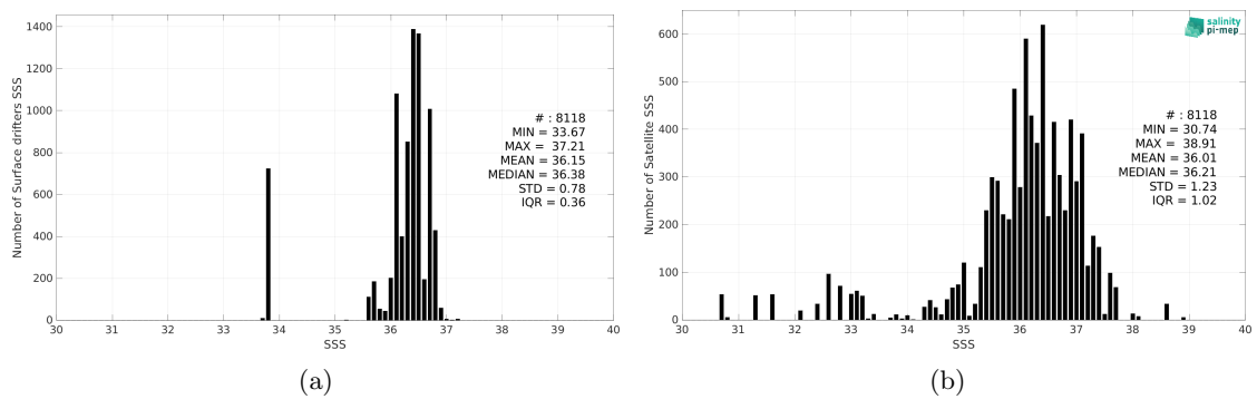
Figure 2: Histograms of SSS from Surface drifters (a) and SMOS SSS L2Q v331 - 0.25 Deg (CATDS-CPDC) (b) considering all match-up pairs per bins of 0.1 over the South Atlantic Ocean Pi-MEP region and for the full satellite product period.
