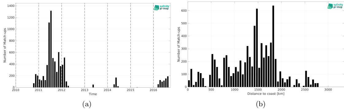
Figure 1: Number of match-ups between Surface drifters and SMOS SSS L2Q v331 - 0.25 Deg (CATDS-CPDC) SSS as a function of time (a) and as function of the distance to coast (b) over the South Atlantic Ocean Pi-MEP region and for the full satellite product period.
