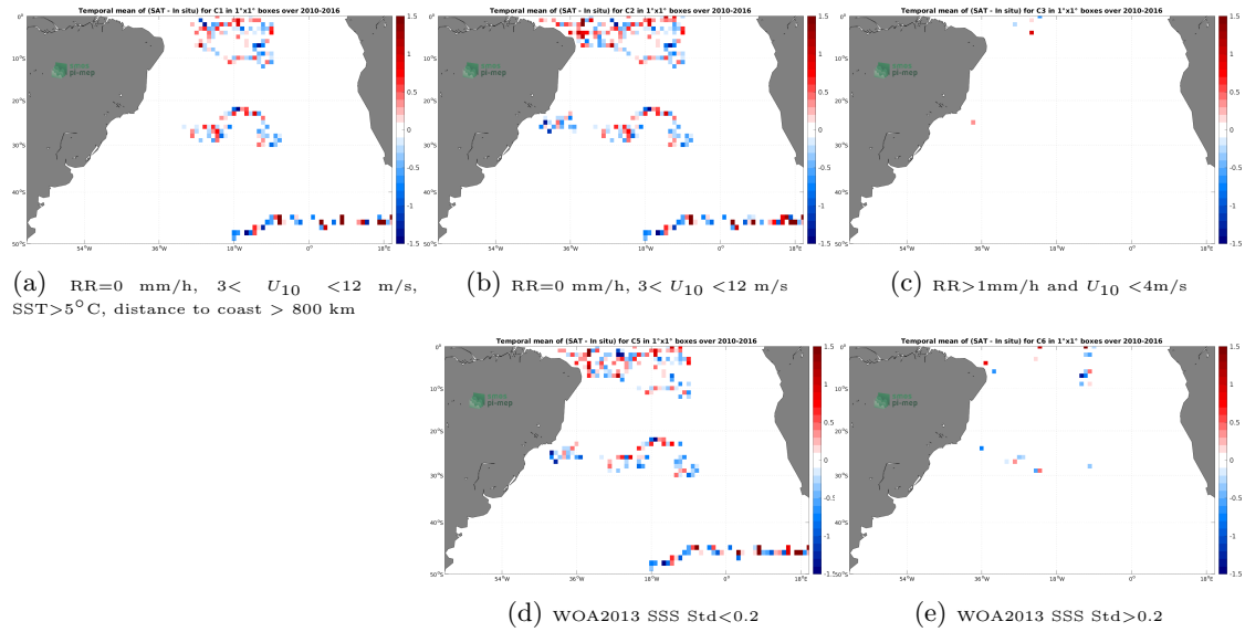
Figure 11: Temporal mean gridded over spatial boxes of size 1^\circ \times 1^\circ of \Delta\text{SSS} (SMOS SSS L2Q v331 - 0.25 Deg (CATDS-CPDC) - Surface drifters) for 5 different subdatasets corresponding to:RR=0 mm/h, 3 < U_{10} < 12 m/s, SST >5^\circ\text{C} , distance to coast > 800 km (a), RR=0 mm/h, 3 < U_{10} < 12 m/s (b), RR >1 mm/h and U_{10} < 4 m/s (c), WOA2013 SSS Std <0.2 (d), WOA2013 SSS Std >0.2 (e).
