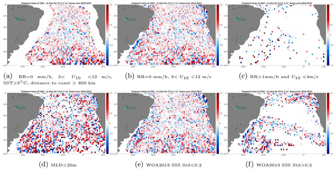
Figure 12: Temporal mean gridded over spatial boxes of size 1^\circ \times 1^\circ of \Delta SSS (SMOS SSS L2Q v331 - 0.25 Deg (CATDS-CPDC) - Argo) for 6 different subdatasets corresponding to:RR=0 mm/h, 3 < U_{10} < 12 m/s, SST >5^\circ C, distance to coast > 800 km (a), RR=0 mm/h, 3 < U_{10} < 12 m/s (b), RR >1 mm/h and U_{10} < 4 m/s (c),MLD <20 m (d),WOA2013 SSS Std <0.2 (e),WOA2013 SSS Std >0.2 (f).
