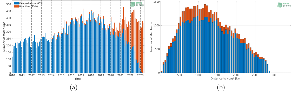
Figure 1: Number of match-ups between Argo and SMOS SSS L2Q v331 - 0.25 Deg (CATDS-CPDC) SSS as a function of time (a) and as function of the distance to coast (b) over the South Atlantic Ocean Pi-MEP region and for the full satellite product period.
