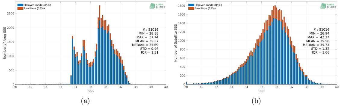
Figure 2: Histograms of SSS from Argo (a) and SMOS SSS L2Q v331 - 0.25 Deg (CATDS-CPDC) (b) considering all match-up pairs per bins of 0.1 over the South Atlantic Ocean Pi-MEP region and for the full satellite product period.
