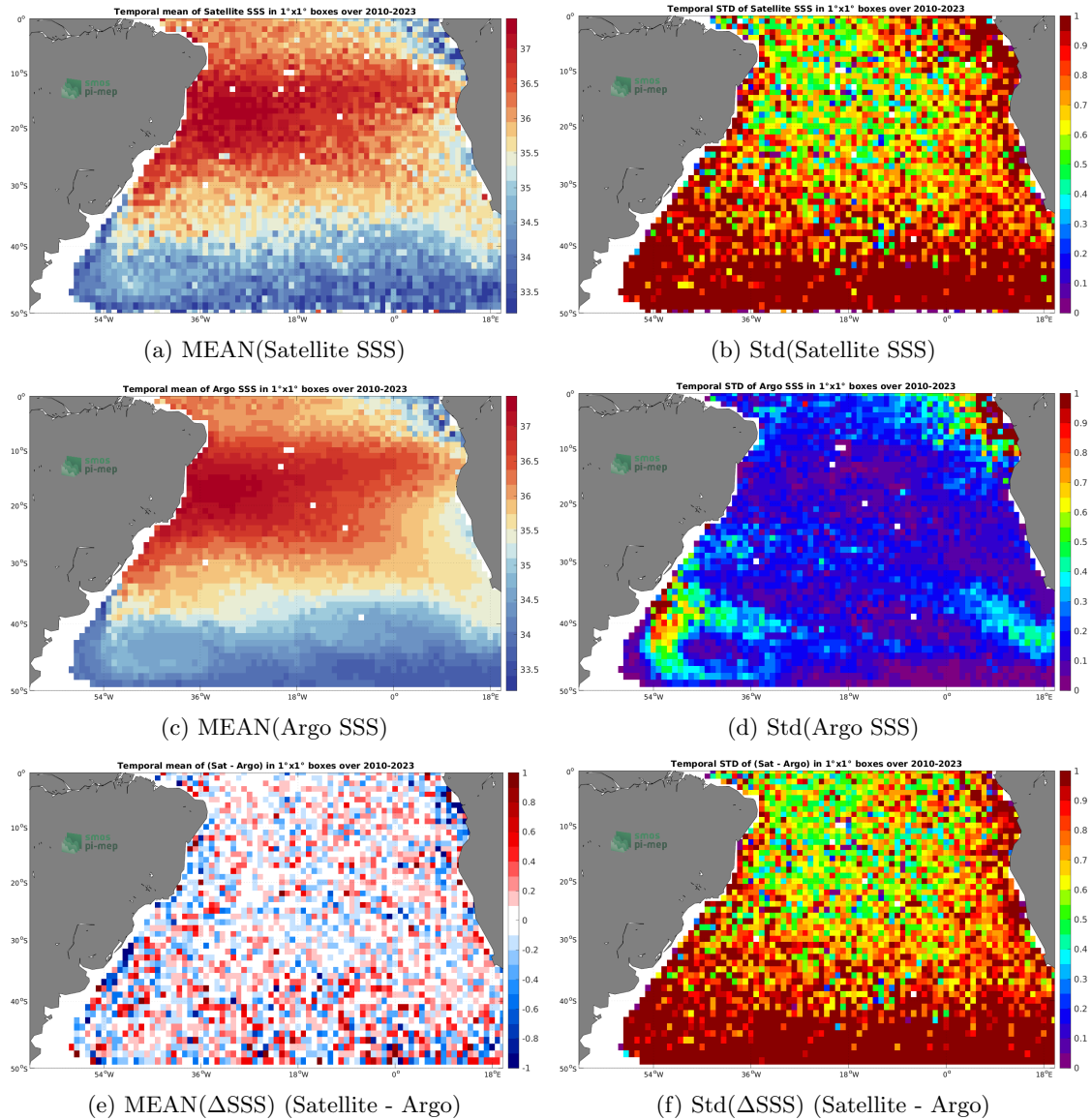
Figure 6: Temporal mean (left) and Std (right) of SSS from SMOS SSS L2Q v331 - 0.25 Deg (CATDS-CPDC) (top), Argo (middle), and of \Delta SSS (Satellite - Argo). Only match-up pairs are used to generate these maps.
