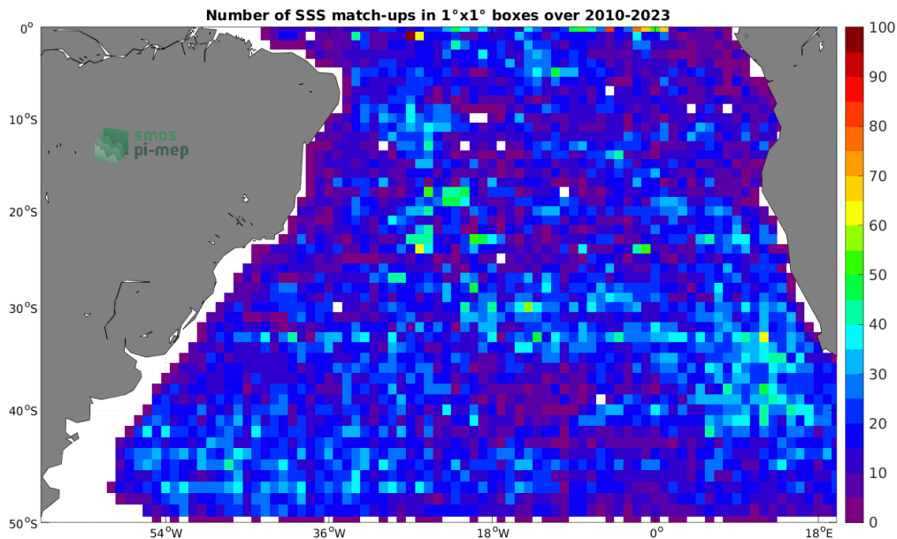
Figure 4: Number of SSS match-ups between Argo SSS and the SMOS SSS L2Q v331 - 0.25 Deg (CATDS-CPDC) SSS product for the South Atlantic Ocean Pi-MEP region over 1^\circ \times 1^\circ boxes and for the full satellite product period.
