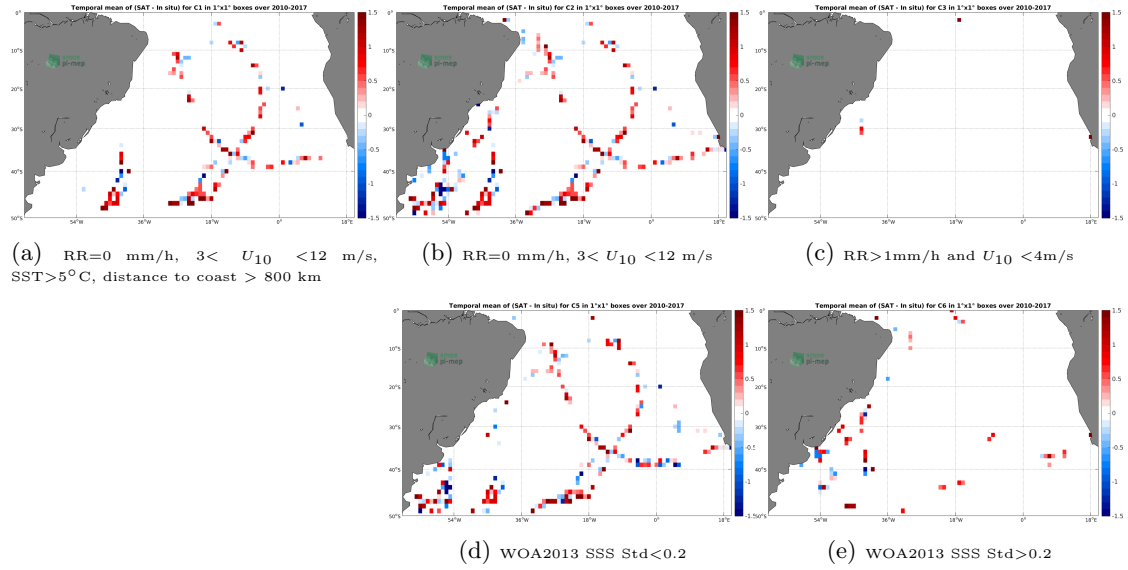
Figure 12: Temporal mean gridded over spatial boxes of size 1^\circ \times 1^\circ of \Delta SSS (SMOS SSS L2Q v330 - 0.25 Deg (CATDS-CPDC) - TSG (GOSUD-Sailing-ship)) for 5 different subdatasets corresponding to: RR=0 mm/h, 3 < U_{10} < 12 m/s, SST > 5^\circ C , distance to coast > 800 km (a), RR=0 mm/h, 3 < U_{10} < 12 m/s (b), RR > 1 mm/h and U_{10} < 4 m/s (c), WOA2013 SSS Std < 0.2 (d), WOA2013 SSS Std > 0.2 (e).
