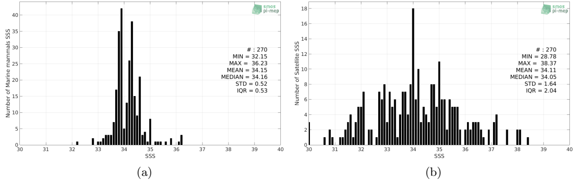
Figure 2: Histograms of SSS from Marine mammals (a) and SMOS SSS L2Q v330 - 0.25 Deg (CATDS-CPDC) (b) considering all match-up pairs per bins of 0.1 over the South Atlantic Ocean Pi-MEP region and for the full satellite product period.
