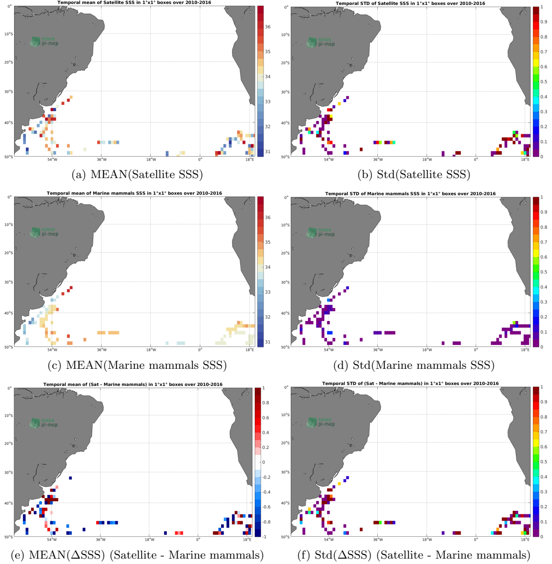
Figure 6: Temporal mean (left) and Std (right) of SSS from SMOS SSS L2Q v330 - 0.25 Deg (CATDS-CPDC) (top), Marine mammals (middle), and of \Delta SSS (Satellite - Marine mammals). Only match-up pairs are used to generate these maps.
