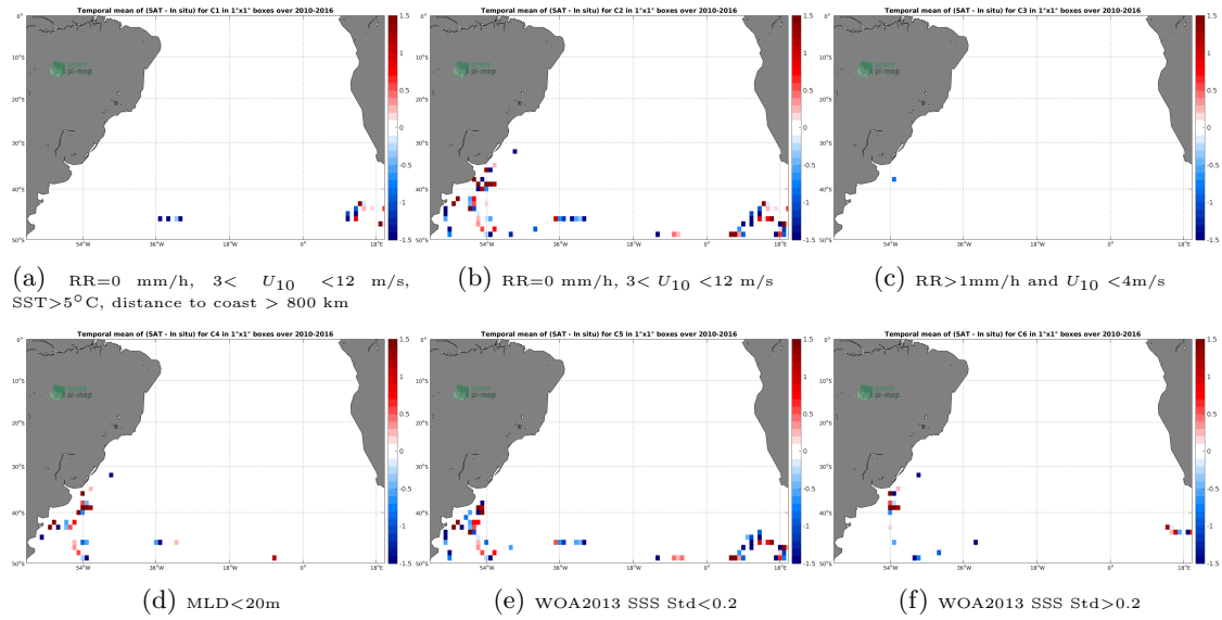
Figure 12: Temporal mean gridded over spatial boxes of size 1^\circ \times 1^\circ of \Delta SSS (SMOS SSS L2Q v330 - 0.25 Deg (CATDS-CPDC) - Marine mammals) for 6 different subdatasets corresponding to: RR=0 mm/h, 3 < U_{10} < 12 m/s, SST > 5^\circ C , distance to coast > 800 km (a), RR=0 mm/h, 3 < U_{10} < 12 m/s (b), RR > 1 mm/h and U_{10} < 4 m/s (c), MLD < 20 m (d), WOA2013 SSS Std < 0.2 (e), WOA2013 SSS Std > 0.2 (f).
