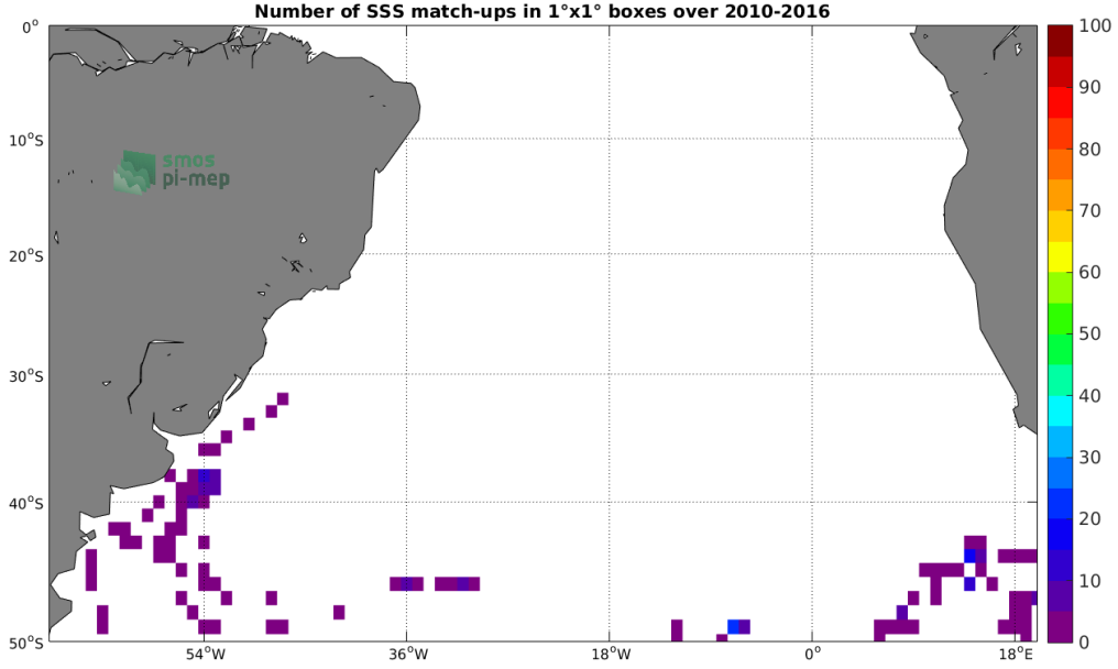
Figure 4: Number of SSS match-ups between Marine mammals SSS and the SMOS SSS L2Q v330 - 0.25 Deg (CATDS-CPDC) SSS product for the South Atlantic Ocean Pi-MEP region over 1^\circ \times 1^\circ boxes and for the full satellite product period.
