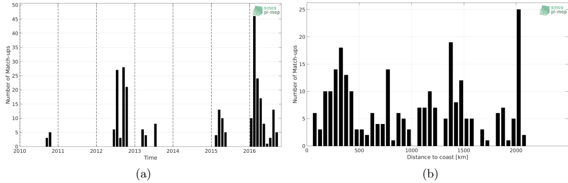
Figure 1: Number of match-ups between Marine mammals and SMOS SSS L2Q v330 - 0.25 Deg (CATDS-CPDC) SSS as a function of time (a) and as function of the distance to coast (b) over the South Atlantic Ocean Pi-MEP region and for the full satellite product period.
