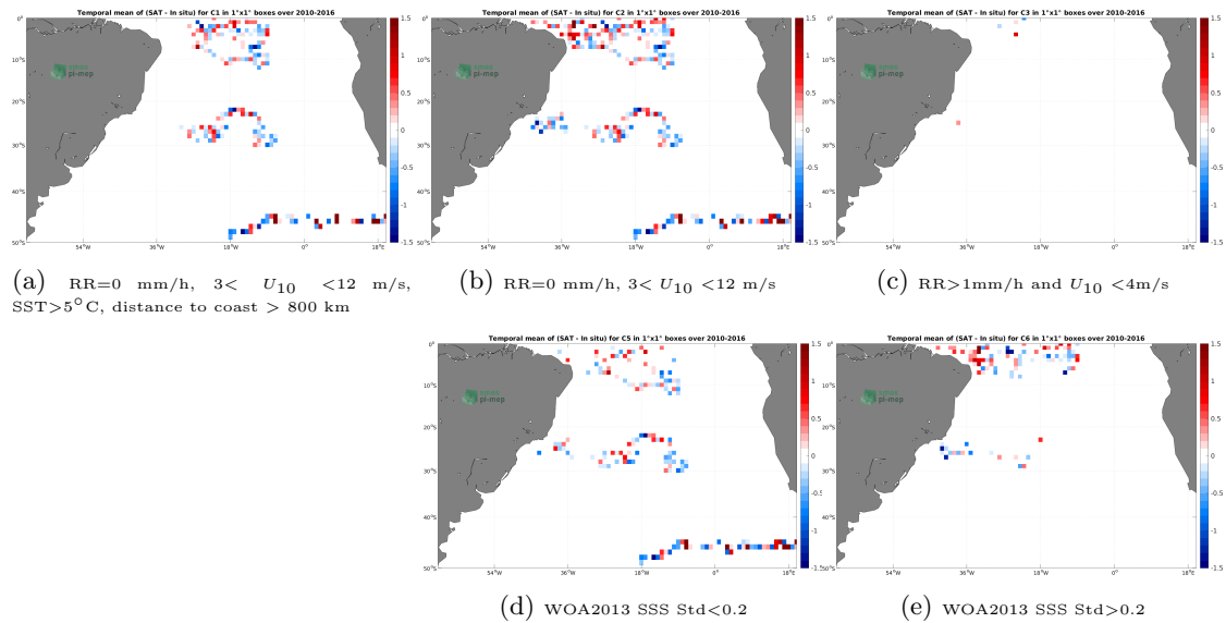
Figure 11: Temporal mean gridded over spatial boxes of size 1^\circ \times 1^\circ of \Delta\text{SSS} (SMOS SSS L2Q v330 - 0.25 Deg (CATDS-CPDC) - Surface drifters) for 5 different subdatasets corresponding to:RR=0 mm/h, 3 < U_{10} < 12 m/s, SST >5^\circ\text{C} , distance to coast > 800 km (a), RR=0 mm/h, 3 < U_{10} < 12 m/s (b), RR >1 mm/h and U_{10} < 4 m/s (c), WOA2013 SSS Std <0.2 (d), WOA2013 SSS Std >0.2 (e).
