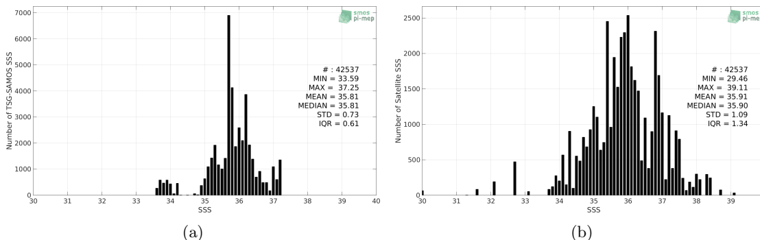
Figure 2: Histograms of SSS from TSG-SAMOS (a) and SMOS L2Q v321 - 0.25 Deg (CATDS-CPDC) (b) considering all match-up pairs per bins of 0.1 over the South Atlantic Ocean Pi-MEP region and for the full satellite product period.
