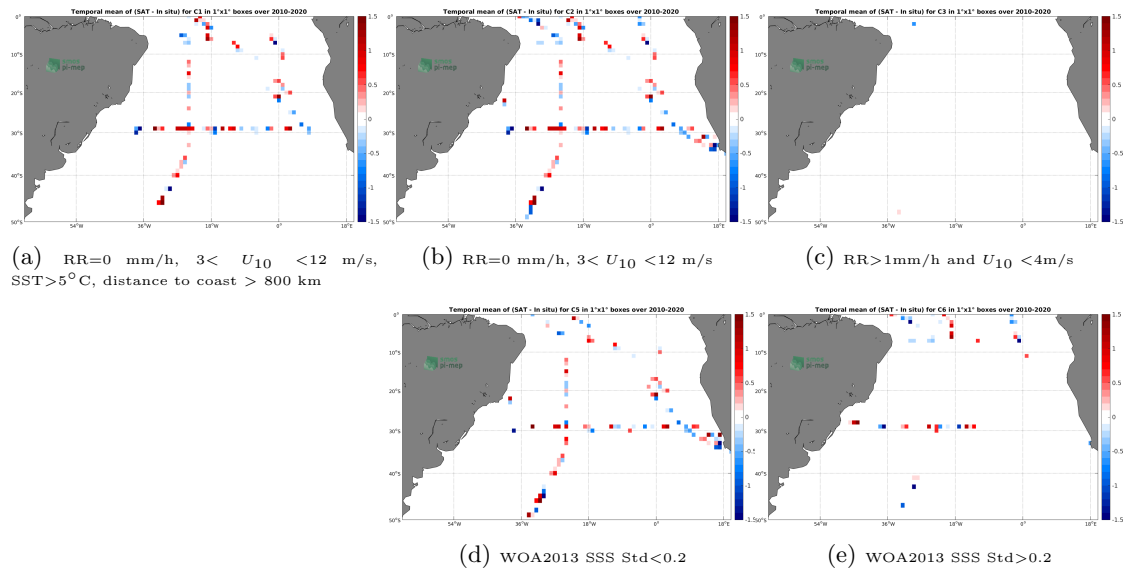
Figure 12: Temporal mean gridded over spatial boxes of size 1^\circ \times 1^\circ of \Delta SSS (SMOS L2Q v321 - 0.25 Deg (CATDS-CPDC) - TSG-SAMOS) for 5 different subdatasets corresponding to:RR=0 mm/h, 3 < U_{10} < 12 m/s, SST >5^\circ C, distance to coast > 800 km (a), RR=0 mm/h, 3 < U_{10} < 12 m/s (b), RR >1 mm/h and U_{10} < 4 m/s (c), WOA2013 SSS Std <0.2 (d), WOA2013 SSS Std >0.2 (e).
