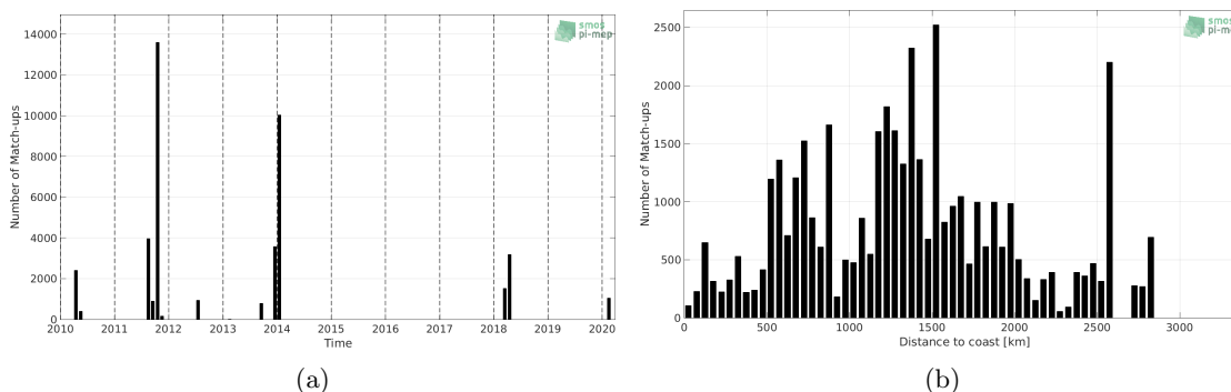
Figure 1: Number of match-ups between TSG-SAMOS and SMOS L2Q v321 - 0.25 Deg (CATDS-CPDC) SSS as a function of time (a) and as function of the distance to coast (b) over the South Atlantic Ocean Pi-MEP region and for the full satellite product period.
