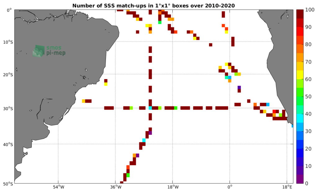
Figure 4: Number of SSS match-ups between TSG-SAMOS SSS and the SMOS L2Q v321 - 0.25 Deg (CATDS-CPDC) SSS product for the South Atlantic Ocean Pi-MEP region over 1^\circ \times 1^\circ boxes and for the full satellite product period.
