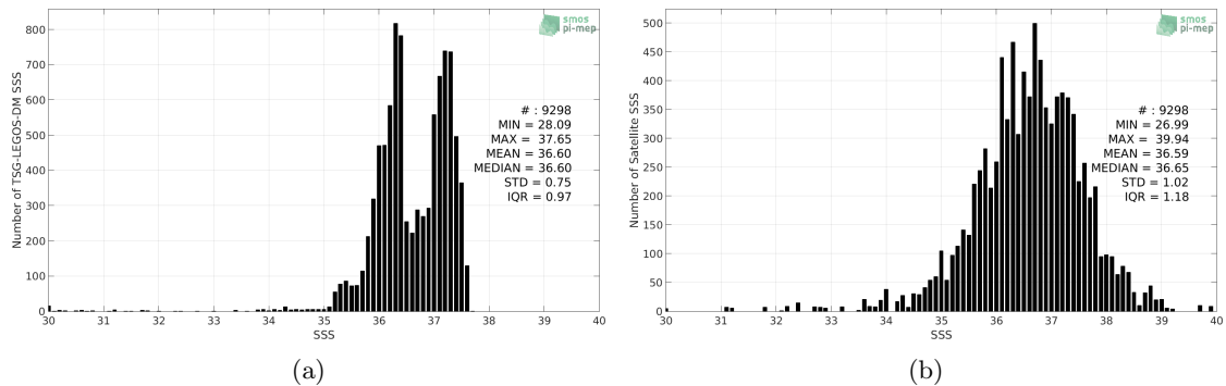
Figure 2: Histograms of SSS from TSG-LEGOS-DM (a) and SMOS-L3-CATDS-CPDC-V321-L2Q (b) considering all match-up pairs per bins of 0.1 over the South Atlantic Ocean Pi-MEP region and for the full satellite product period.
