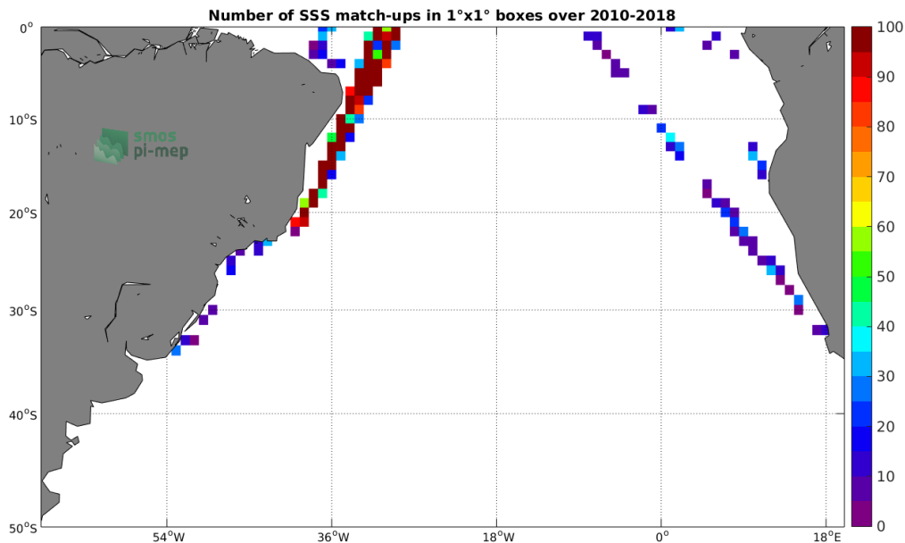
Figure 4: Number of SSS match-ups between TSG-LEGOS-DM SSS and the SMOS-L3-CATDS-CPDC-V321-L2Q SSS product for the South Atlantic Ocean Pi-MEP region over 1^\circ \times 1^\circ boxes and for the full satellite product period.
