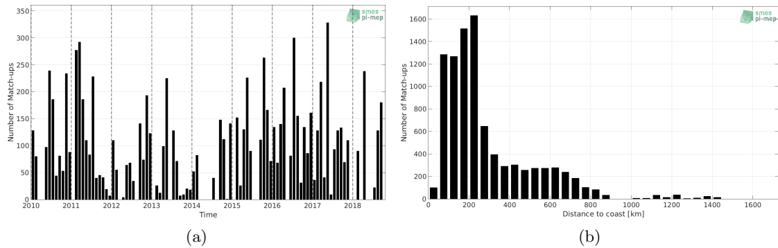
Figure 1: Number of match-ups between TSG-LEGOS-DM and SMOS-L3-CATDS-CPDC-V321-L2Q SSS as a function of time (a) and as function of the distance to coast (b) over the South Atlantic Ocean Pi-MEP region and for the full satellite product period.
