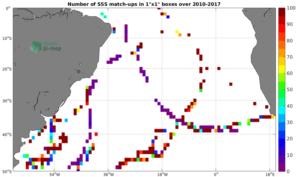
Figure 4: Number of SSS match-ups between TSG (GOSUD-Sailing-ship) SSS and the SMOS SSS L2Q v321 - 0.25 Deg (CATDS-CPDC) SSS product for the South Atlantic Ocean Pi-MEP region over 1^{\circ} \times 1^{\circ} boxes and for the full satellite product period.
