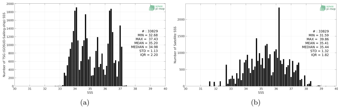
Figure 2: Histograms of SSS from TSG (GOSUD-Sailing-ship) (a) and SMOS SSS L2Q v321 - 0.25 Deg (CATDS-CPDC) (b) considering all match-up pairs per bins of 0.1 over the South Atlantic Ocean Pi-MEP region and for the full satellite product period.
