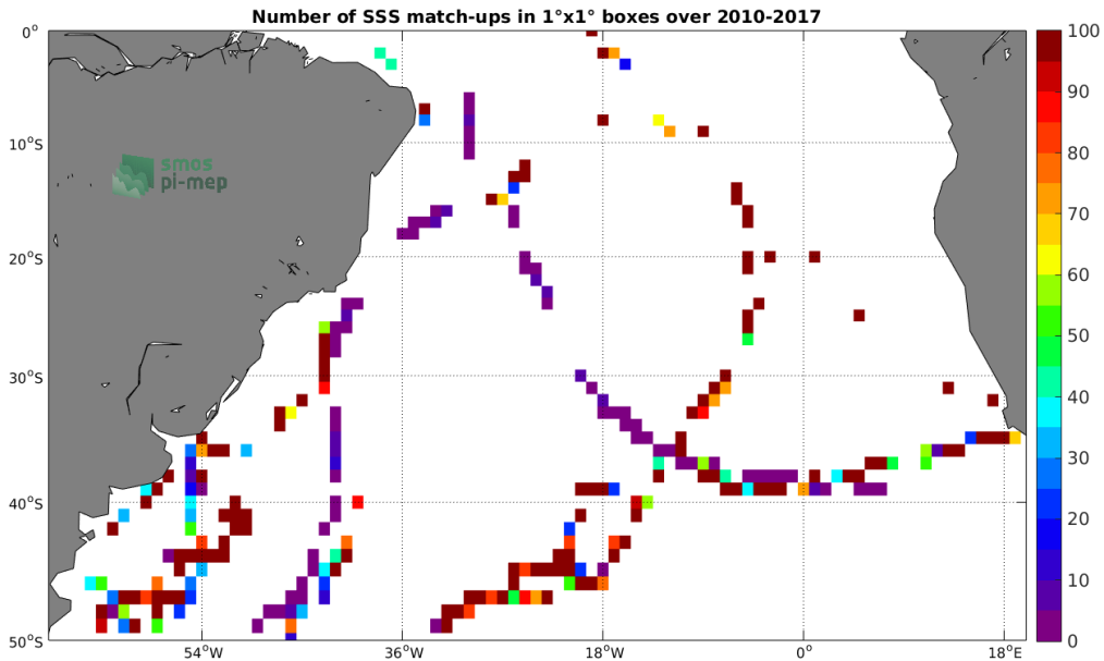
Figure 4: Number of SSS match-ups between TSG (GOSUD-Sailing-ship) SSS and the SMOS SSS L2Q v321 - 0.25 Deg (CATDS-CPDC) SSS product for the South Atlantic Ocean Pi-MEP region over 1^\circ \times 1^\circ boxes and for the full satellite product period.
