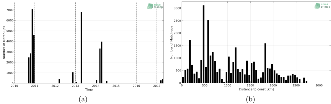
Figure 1: Number of match-ups between TSG (GOSUD-Sailing-ship) and SMOS SSS L2Q v321 - 0.25 Deg (CATDS-CPDC) SSS as a function of time (a) and as function of the distance to coast (b) over the South Atlantic Ocean Pi-MEP region and for the full satellite product period.
