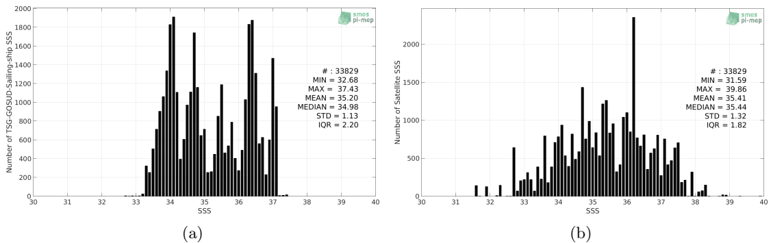
Figure 2: Histograms of SSS from TSG-GOSUD-Sailing-ship (a) and SMOS L2Q v321 - 0.25 Deg (CATDS-CPDC) (b) considering all match-up pairs per bins of 0.1 over the South Atlantic Ocean Pi-MEP region and for the full satellite product period.
