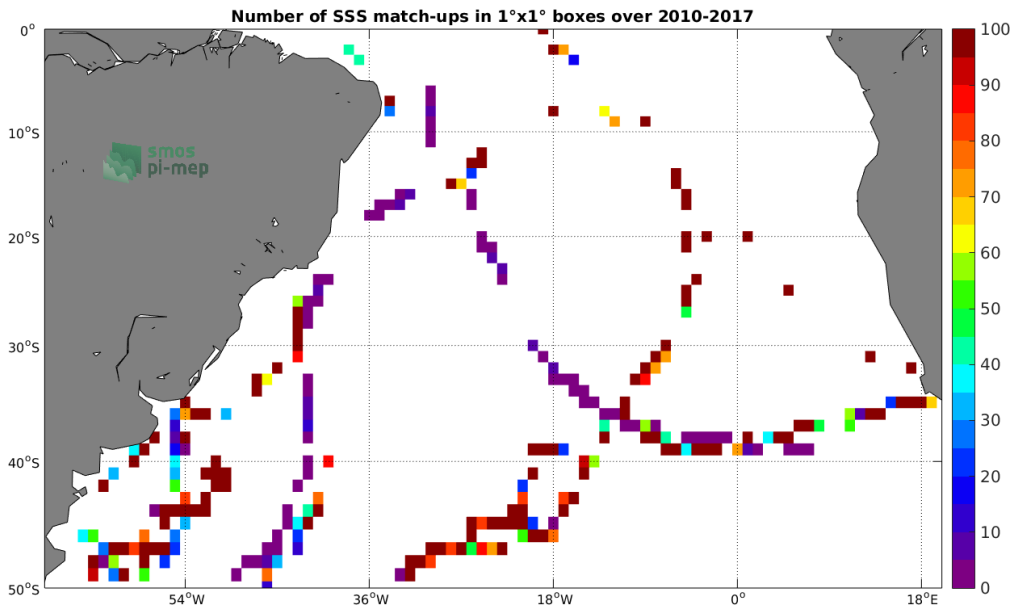
Figure 4: Number of SSS match-ups between TSG-GOSUD-Sailing-ship SSS and the SMOS L2Q v321 - 0.25 Deg (CATDS-CPDC) SSS product for the South Atlantic Ocean Pi-MEP region over 1^\circ \times 1^\circ boxes and for the full satellite product period.
