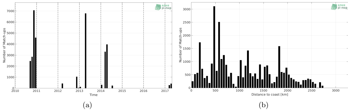
Figure 1: Number of match-ups between TSG-GOSUD-Sailing-ship and SMOS L2Q v321 - 0.25 Deg (CATDS-CPDC) SSS as a function of time (a) and as function of the distance to coast (b) over the South Atlantic Ocean Pi-MEP region and for the full satellite product period.
