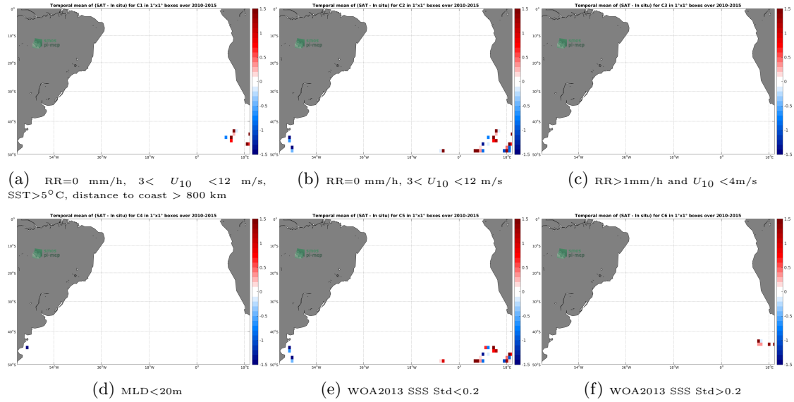
Figure 12: Temporal mean gridded over spatial boxes of size 1^{\circ} \times 1^{\circ} of \Delta\text{SSS} (SMOS SSS L2Q v321 - 0.25 Deg (CATDS-CPDC) - Marine mammals) for 6 different subdatasets corresponding to:RR=0 mm/h, 3 < U_{10} < 12 m/s, SST >5^{\circ}\text{C} , distance to coast > 800 km (a), RR=0 mm/h, 3 < U_{10} < 12 m/s (b), RR >1\text{mm/h} and U_{10} < 4\text{m/s} (c),MLD <20\text{m} (d),WOA2013 SSS Std <0.2 (e),WOA2013 SSS Std >0.2 (f).
