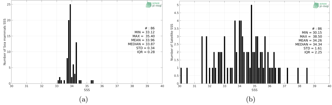
Figure 2: Histograms of SSS from Marine mammals (a) and SMOS SSS L2Q v321 - 0.25 Deg (CATDS-CPDC) (b) considering all match-up pairs per bins of 0.1 over the South Atlantic Ocean Pi-MEP region and for the full satellite product period.
