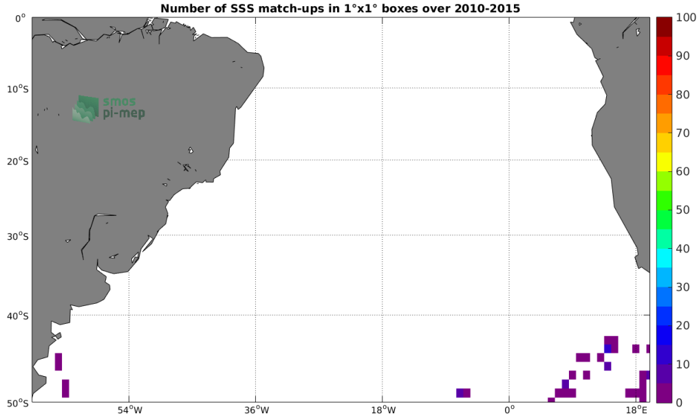
Figure 4: Number of SSS match-ups between Marine mammals SSS and the SMOS SSS L2Q v321 - 0.25 Deg (CATDS-CPDC) SSS product for the South Atlantic Ocean Pi-MEP region over 1^\circ \times 1^\circ boxes and for the full satellite product period.
