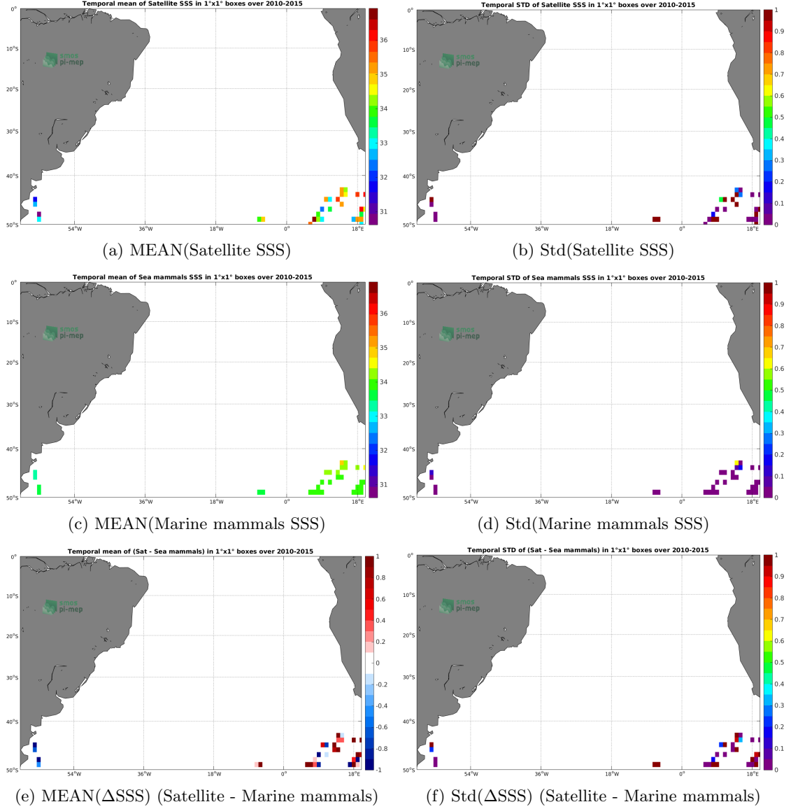
Figure 6: Temporal mean (left) and Std (right) of SSS from SMOS SSS L2Q v321 - 0.25 Deg (CATDS-CPDC) (top), Marine mammals (middle), and of \Delta SSS (Satellite - Marine mammals). Only match-up pairs are used to generate these maps.
