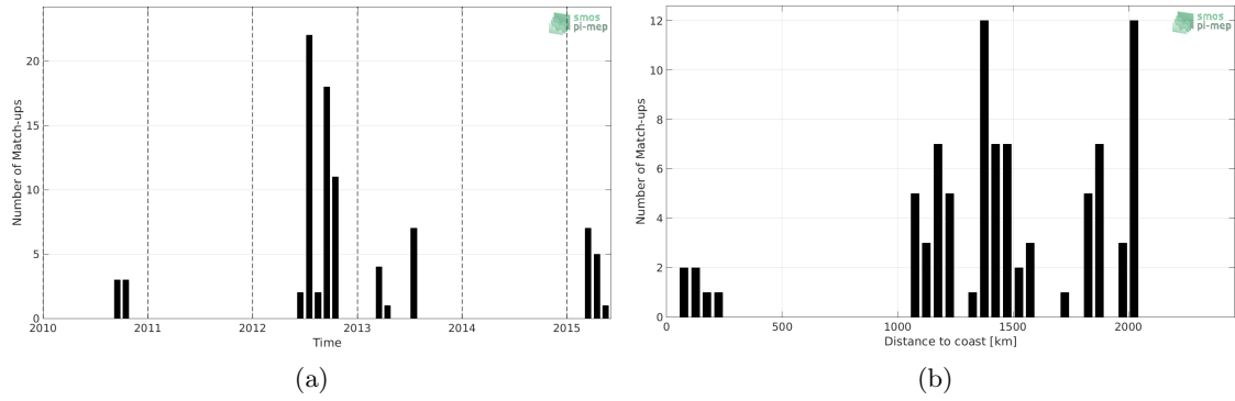
Figure 1: Number of match-ups between Marine mammals and SMOS SSS L2Q v321 - 0.25 Deg (CATDS-CPDC) SSS as a function of time (a) and as function of the distance to coast (b) over the South Atlantic Ocean Pi-MEP region and for the full satellite product period.
