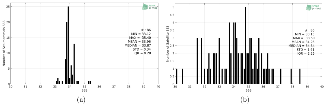
Figure 2: Histograms of SSS from Sea mammals (a) and SMOS SSS L2Q v321 - 0.25 Deg (CATDS-CPDC) (b) considering all match-up pairs per bins of 0.1 over the South Atlantic Ocean Pi-MEP region and for the full satellite product period.
