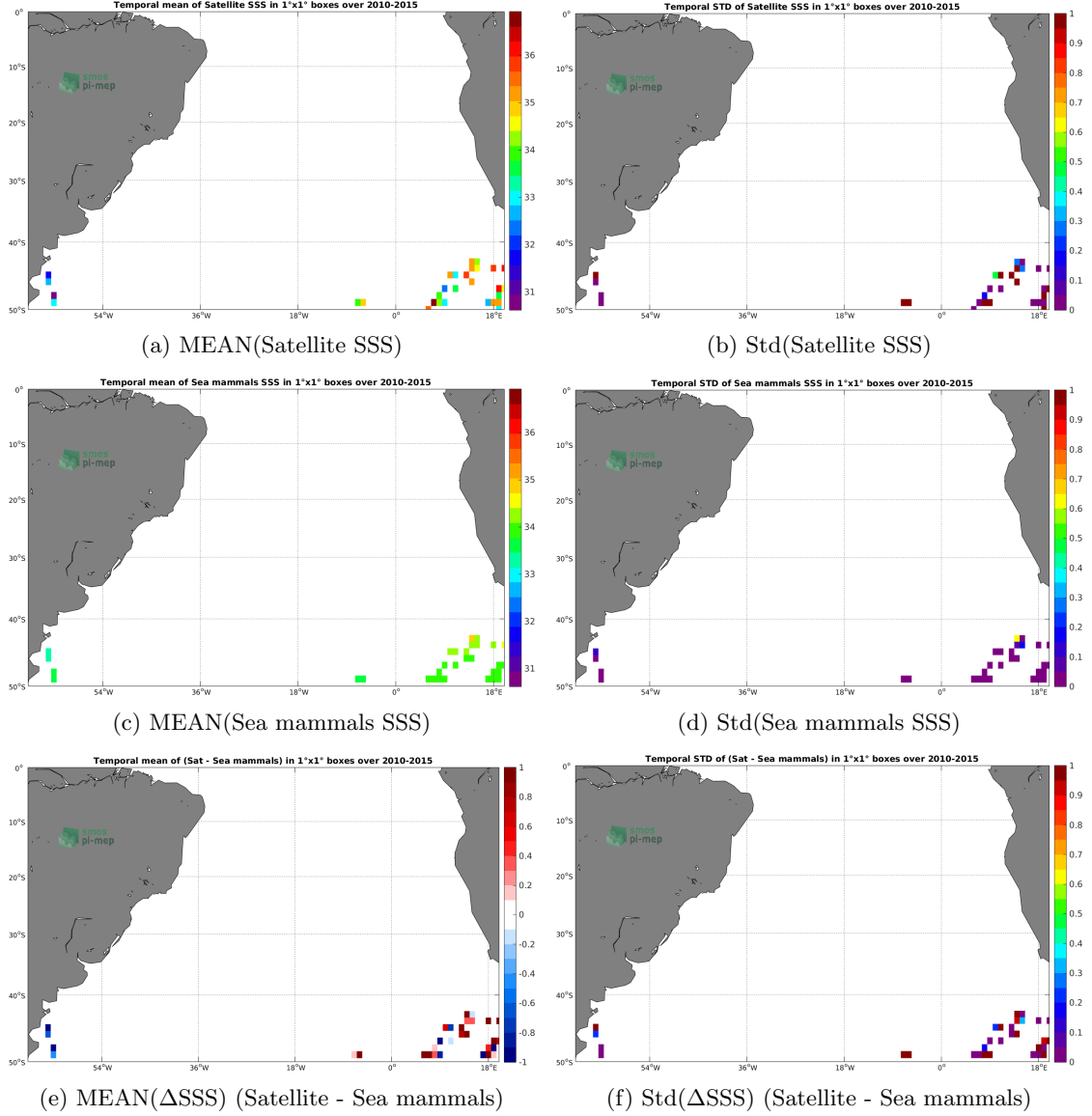
Figure 6: Temporal mean (left) and Std (right) of SSS from SMOS SSS L2Q v321 - 0.25 Deg (CATDS-CPDC) (top), Sea mammals (middle), and of \Delta SSS (Satellite - Sea mammals). Only match-up pairs are used to generate these maps.
