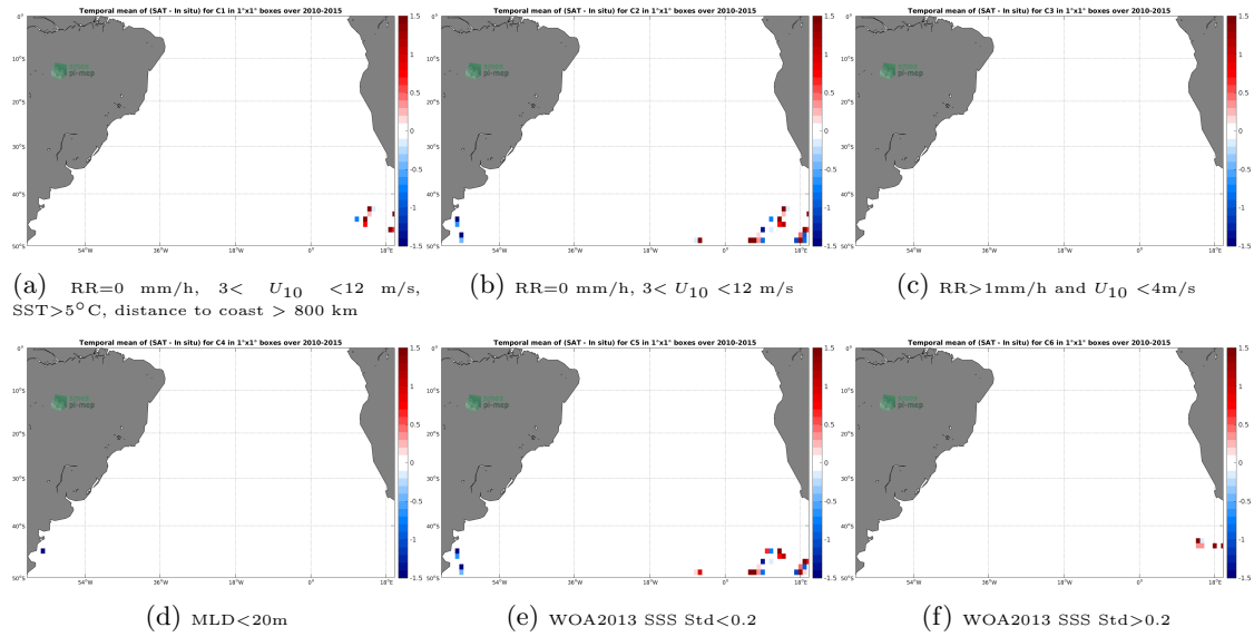
Figure 12: Temporal mean gridded over spatial boxes of size 1^{\circ}\times 1^{\circ} of \Delta\text{SSS} (SMOS SSS L2Q v321 - 0.25 Deg (CATDS-CPDC) - Sea mammals) for 6 different subdatasets corresponding to:RR=0 mm/h, 3 < U_{10} < 12 m/s, SST >5^{\circ}\text{C} , distance to coast > 800 km (a), RR=0 mm/h, 3 < U_{10} < 12 m/s (b), RR >1\text{mm/h} and U_{10} < 4\text{m/s} (c),MLD <20\text{m} (d),WOA2013 SSS Std <0.2 (e),WOA2013 SSS Std >0.2 (f).
