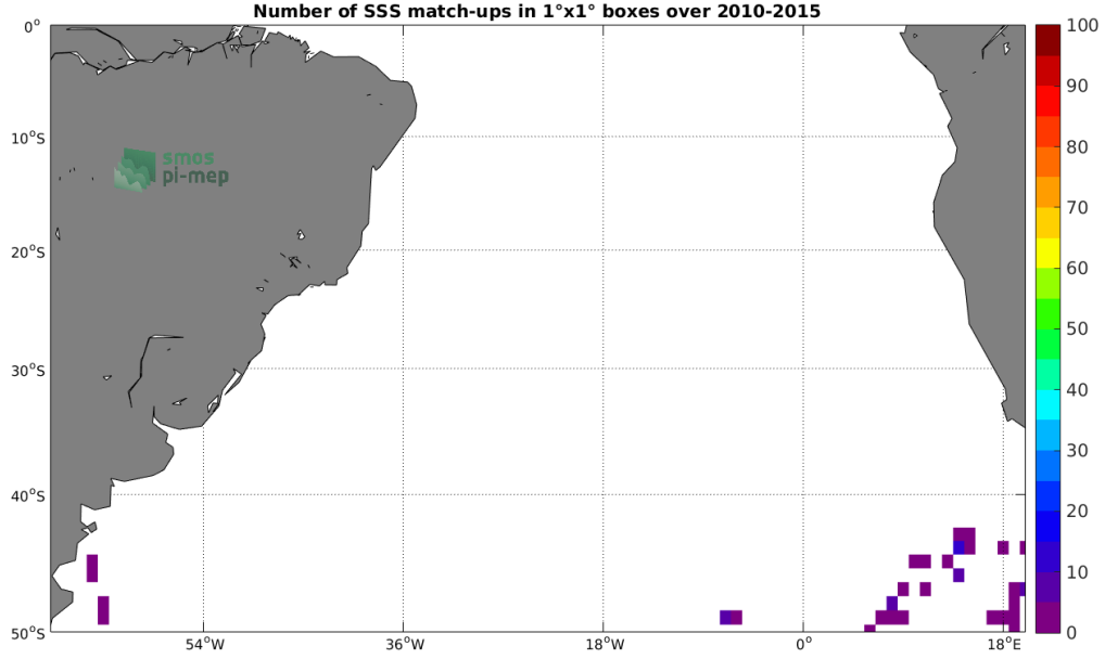
Figure 4: Number of SSS match-ups between Sea mammals SSS and the SMOS SSS L2Q v321 - 0.25 Deg (CATDS-CPDC) SSS product for the South Atlantic Ocean Pi-MEP region over 1°x1° boxes and for the full satellite product period.
