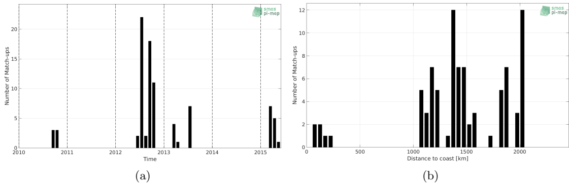
Figure 1: Number of match-ups between Sea mammals and SMOS SSS L2Q v321 - 0.25 Deg (CATDS-CPDC) SSS as a function of time (a) and as function of the distance to coast (b) over the South Atlantic Ocean Pi-MEP region and for the full satellite product period.
