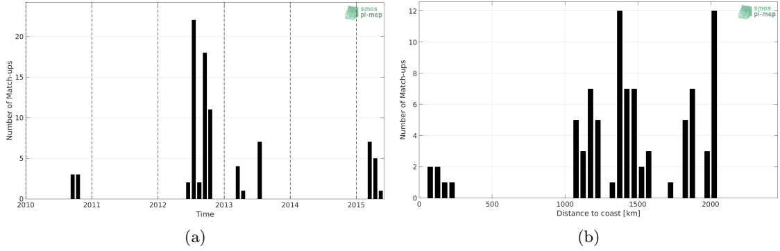
Figure 1: Number of match-ups between Sea mammals and SMOS SSS L2Q v321 - 0.25 Deg (CATDS-CPDC) SSS as a function of time (a) and as function of the distance to coast (b) over the South Atlantic Ocean Pi-MEP region and for the full satellite product period.
