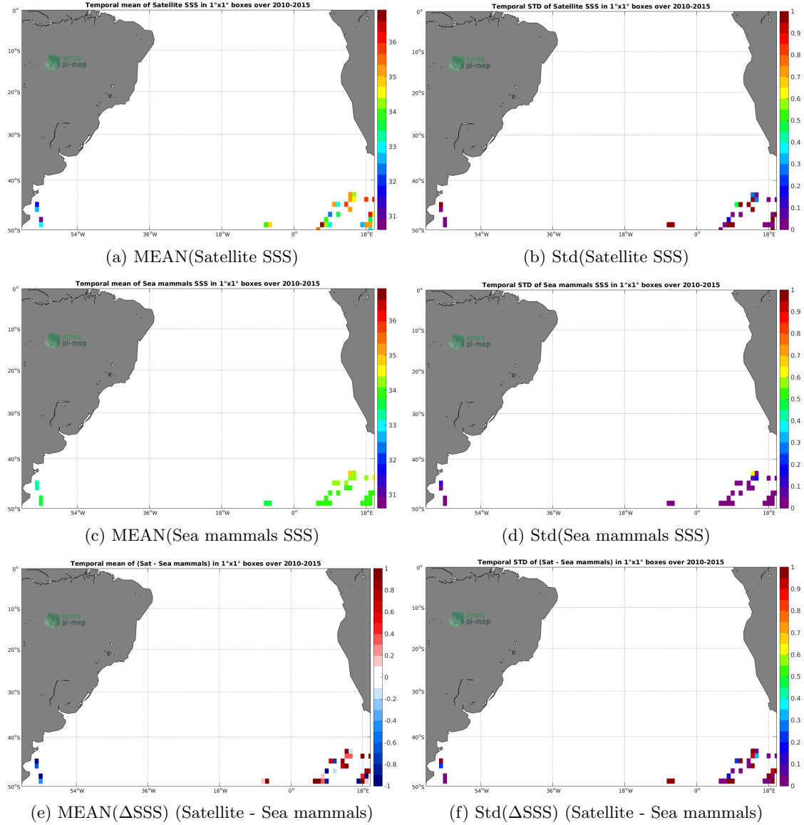
Figure 6: Temporal mean (left) and Std (right) of SSS from SMOS L2Q v321 - 0.25 Deg (CATDS-CPDC) (top), Sea mammals (middle), and of \Delta SSS (Satellite - Sea mammals). Only match-up pairs are used to generate these maps.
