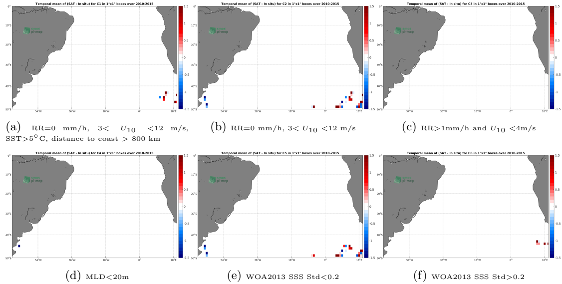
Figure 12: Temporal mean gridded over spatial boxes of size 1^{\circ}\times 1^{\circ} of \Delta\text{SSS} (SMOS L2Q v321 - 0.25 Deg (CATDS-CPDC) - Sea mammals) for 6 different subdatasets corresponding to:RR=0 mm/h, 3 < U_{10} < 12 m/s, SST >5^{\circ}\text{C} , distance to coast > 800 km (a), RR=0 mm/h, 3 < U_{10} < 12 m/s (b), RR >1 mm/h and U_{10} < 4 m/s (c),MLD <20 m (d),WOA2013 SSS Std <0.2 (e),WOA2013 SSS Std >0.2 (f).
