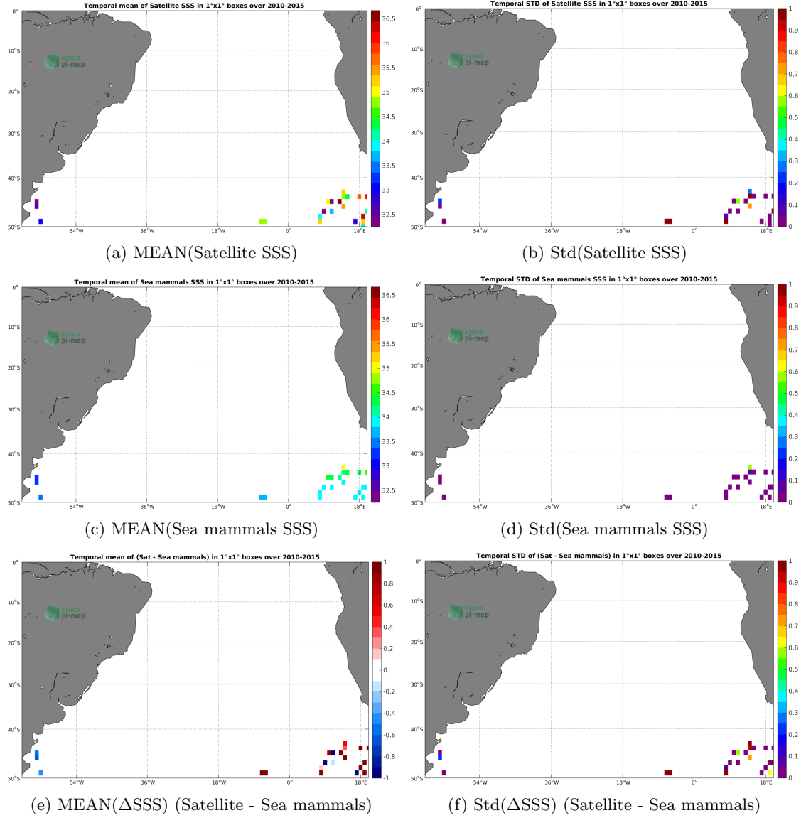
Figure 6: Temporal mean (left) and Std (right) of SSS from SMOS-L3-CATDS-CPDC-V321-L2Q (top), Sea mammals (middle), and of \Delta SSS (Satellite - Sea mammals). Only match-up pairs are used to generate these maps.
