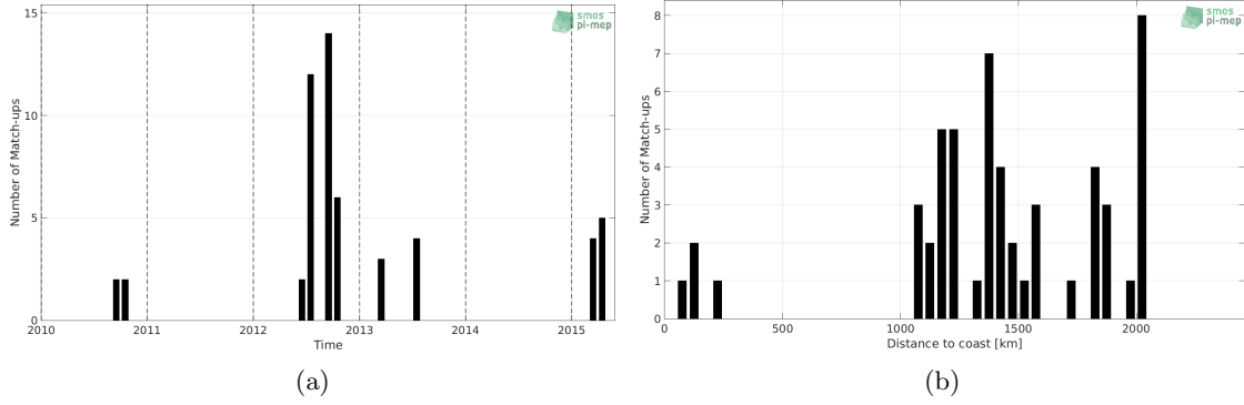
Figure 1: Number of match-ups between Sea mammals and SMOS-L3-CATDS-CPDC-V321-L2Q SSS as a function of time (a) and as function of the distance to coast (b) over the South Atlantic Ocean Pi-MEP region and for the full satellite product period.
