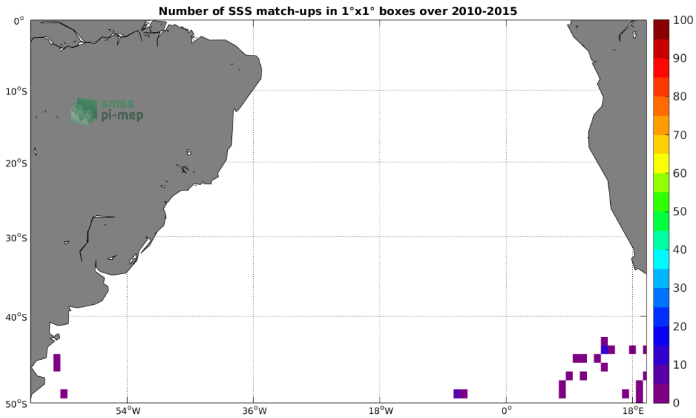
Figure 4: Number of SSS match-ups between Sea mammals SSS and the SMOS-L3-CATDS-CPDC-V321-L2Q SSS product for the South Atlantic Ocean Pi-MEP region over 1°x1° boxes and for the full satellite product period.
