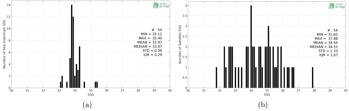
Figure 2: Histograms of SSS from Sea mammals (a) and SMOS-L3-CATDS-CPDC-V321-L2Q (b) considering all match-up pairs per bins of 0.1 over the South Atlantic Ocean Pi-MEP region and for the full satellite product period.
