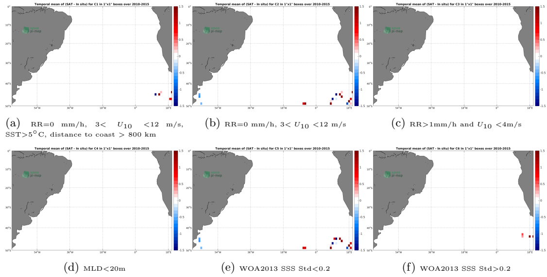
Figure 12: Temporal mean gridded over spatial boxes of size 1^\circ \times 1^\circ of \Delta SSS (SMOS-L3-CATDS-CPDC-V321-L2Q - Sea mammals) for 6 different subdatasets corresponding to: RR=0 mm/h, 3 < U_{10} < 12 m/s, SST > 5^\circ C , distance to coast > 800 km (a), RR=0 mm/h, 3 < U_{10} < 12 m/s (b), RR > 1 mm/h and U_{10} < 4 m/s (c), MLD < 20 m (d), WOA2013 SSS Std < 0.2 (e), WOA2013 SSS Std > 0.2 (f).
