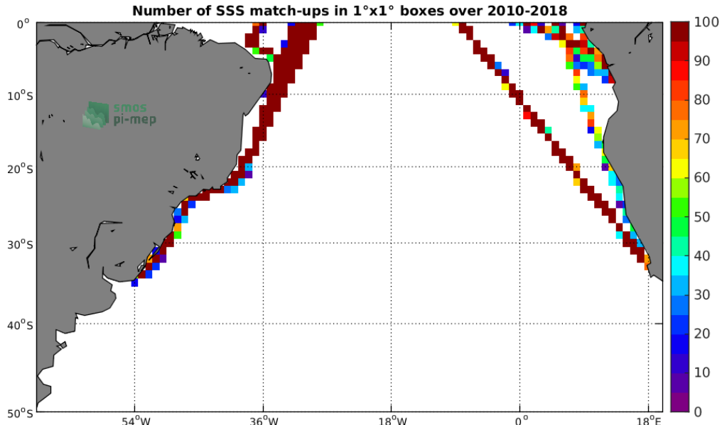
Figure 4: Number of SSS match-ups between TSG-LEGOS-DM SSS and the SMOS-L3-CATDS-CPDC-V317-MONTHLY-25KM SSS product for the South Atlantic Ocean Pi-MEP region over 1^\circ \times 1^\circ boxes and for the full satellite product period.
