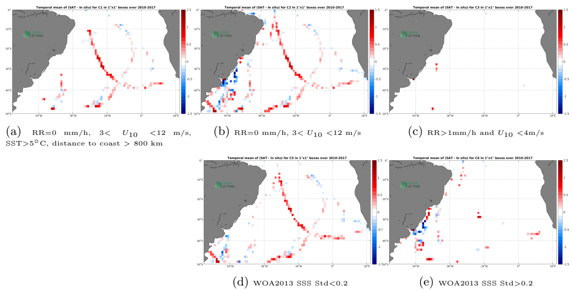
Figure 12: Temporal mean gridded over spatial boxes of size 1^\circ \times 1^\circ of \Delta\text{SSS} (SMOS SSS L3 v317 - Monthly - 25 km (CATDS-CPDC) - TSG (GOSUD-Sailing-ship)) for 5 different subdatasets corresponding to: RR=0 mm/h, 3 < U_{10} < 12 m/s, SST > 5°C, distance to coast > 800 km (a), RR=0 mm/h, 3 < U_{10} < 12 m/s (b), RR > 1mm/h and U_{10} < 4 m/s (c), WOA2013 SSS Std < 0.2 (d), WOA2013 SSS Std > 0.2 (e).
