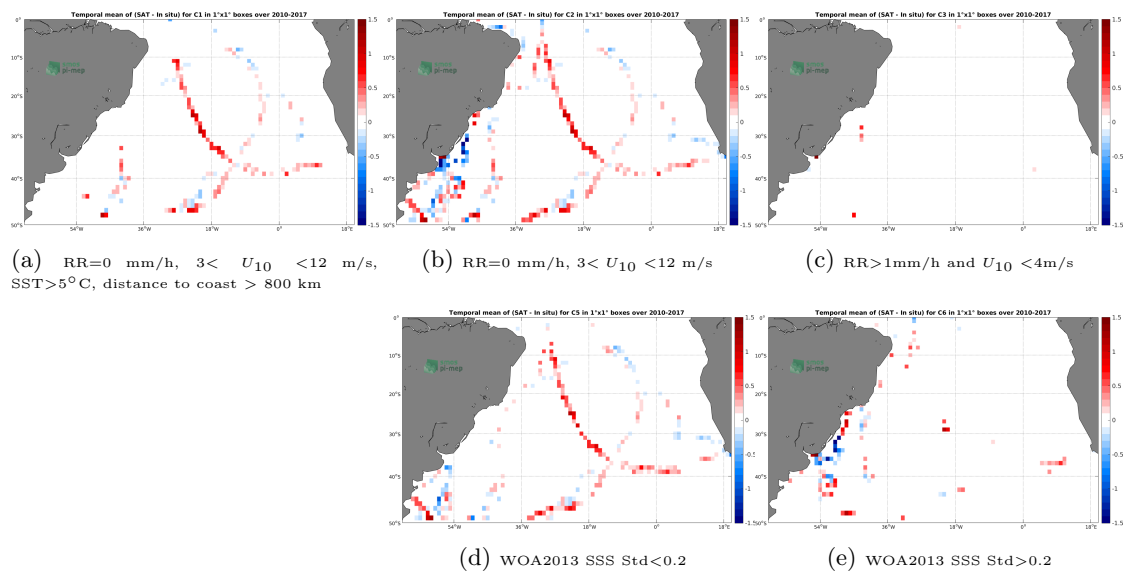
Figure 12: Temporal mean gridded over spatial boxes of size 1^\circ \times 1^\circ of \Delta SSS (SMOS SSS L3 v317 - Monthly - 25 km (CATDS-CPDC) - TSG (GOSUD-Sailing-ship)) for 5 different subdatasets corresponding to:RR=0 mm/h, 3 < U_{10} < 12 m/s, SST>5°C, distance to coast > 800 km (a), RR=0 mm/h, 3 < U_{10} < 12 m/s (b), RR>1mm/h and U_{10} < 4 m/s (c), WOA2013 SSS Std<0.2 (d), WOA2013 SSS Std>0.2 (e).
