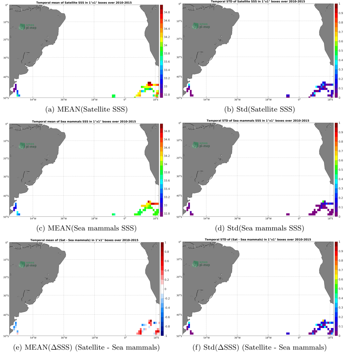
Figure 6: Temporal mean (left) and Std (right) of SSS from SMOS SSS L3 v317 - Monthly - 25 km (CATDS-CPDC) (top), Sea mammals (middle), and of \Delta SSS (Satellite - Sea mammals). Only match-up pairs are used to generate these maps.
