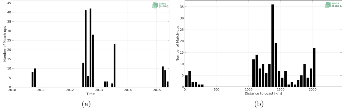
Figure 1: Number of match-ups between Sea mammals and SMOS SSS L3 v317 - Monthly - 25 km (CATDS-CPDC) SSS as a function of time (a) and as function of the distance to coast (b) over the South Atlantic Ocean Pi-MEP region and for the full satellite product period.
