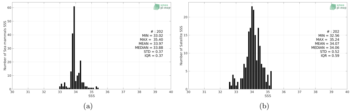
Figure 2: Histograms of SSS from Sea mammals (a) and SMOS SSS L3 v317 - Monthly - 25 km (CATDS-CPDC) (b) considering all match-up pairs per bins of 0.1 over the South Atlantic Ocean Pi-MEP region and for the full satellite product period.
