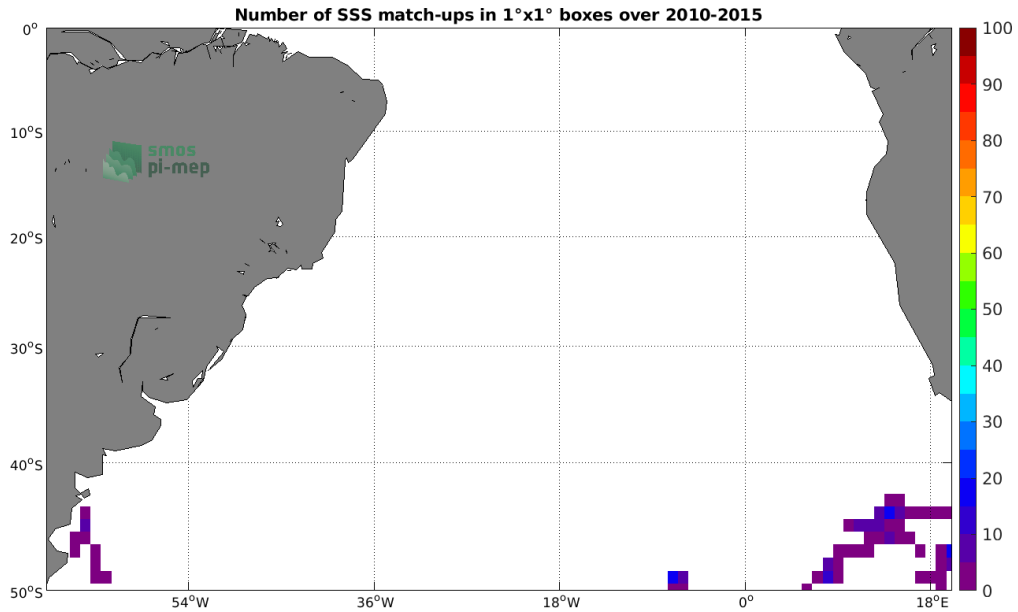
Figure 4: Number of SSS match-ups between Sea mammals SSS and the SMOS SSS L3 v317 - Monthly - 25 km (CATDS-CPDC) SSS product for the South Atlantic Ocean Pi-MEP region over 1°x1° boxes and for the full satellite product period.
