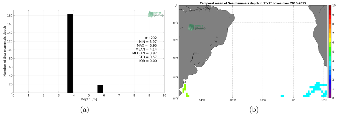
Figure 3: Histograms of the depth of the upper level SSS measurements from Sea mammals in the Match-up DataBase for the South Atlantic Ocean Pi-MEP region (a) and temporal mean spatial distribution of pressure of the in situ SSS data over 1°x1° boxes and for the full satellite product period (b).
