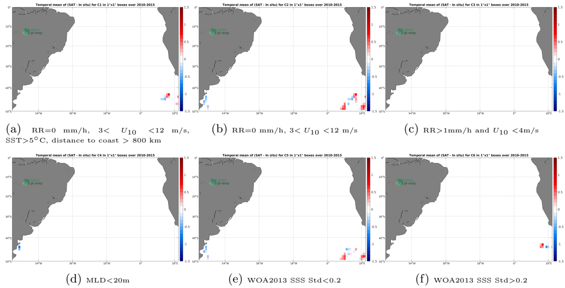
Figure 12: Temporal mean gridded over spatial boxes of size 1^{\circ}\times 1^{\circ} of \Delta\text{SSS} (SMOS SSS L3 v317 - Monthly - 25 km (CATDS-CPDC) - Sea mammals) for 6 different subdatasets corresponding to: \text{RR}=0 mm/h, 3 < U_{10} < 12 m/s, SST > 5^{\circ}\text{C} , distance to coast > 800 km (a), \text{RR}=0 mm/h, 3 < U_{10} < 12 m/s (b), \text{RR} > 1\text{mm/h} and U_{10} < 4\text{m/s} (c), \text{MLD} < 20\text{m} (d), WOA2013 SSS Std < 0.2 (e), WOA2013 SSS Std > 0.2 (f).
