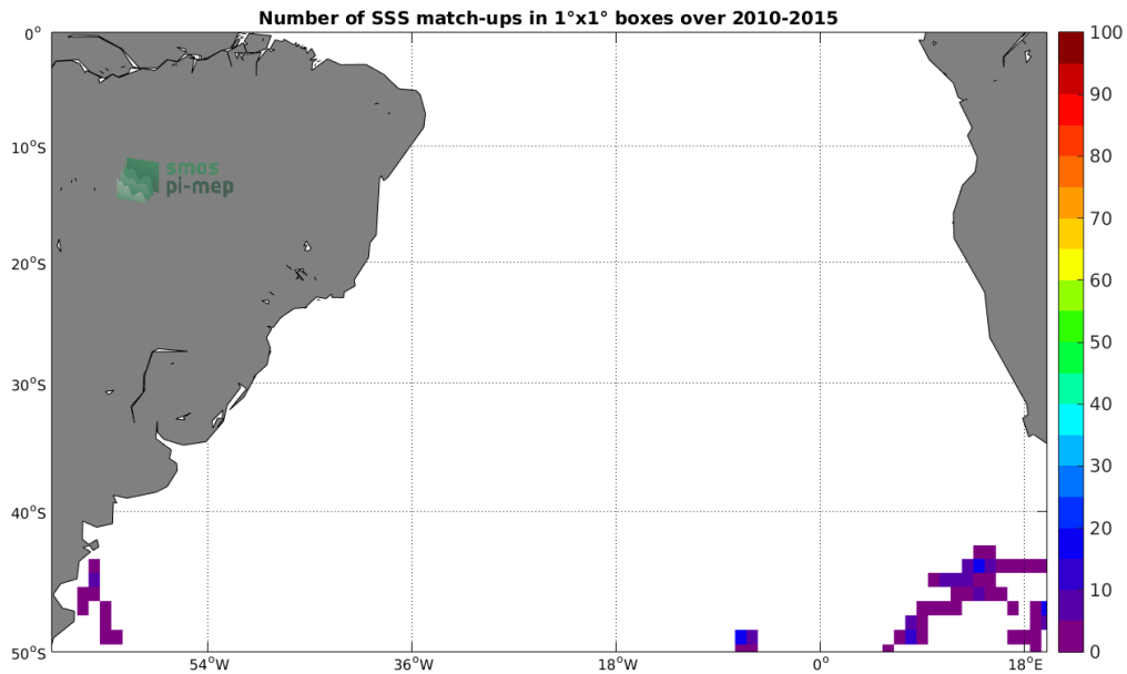
Figure 4: Number of SSS match-ups between Sea mammals SSS and the SMOS L3 v317 - Monthly - 25 km (CATDS-CPDC) SSS product for the South Atlantic Ocean Pi-MEP region over 1°x1° boxes and for the full satellite product period.
