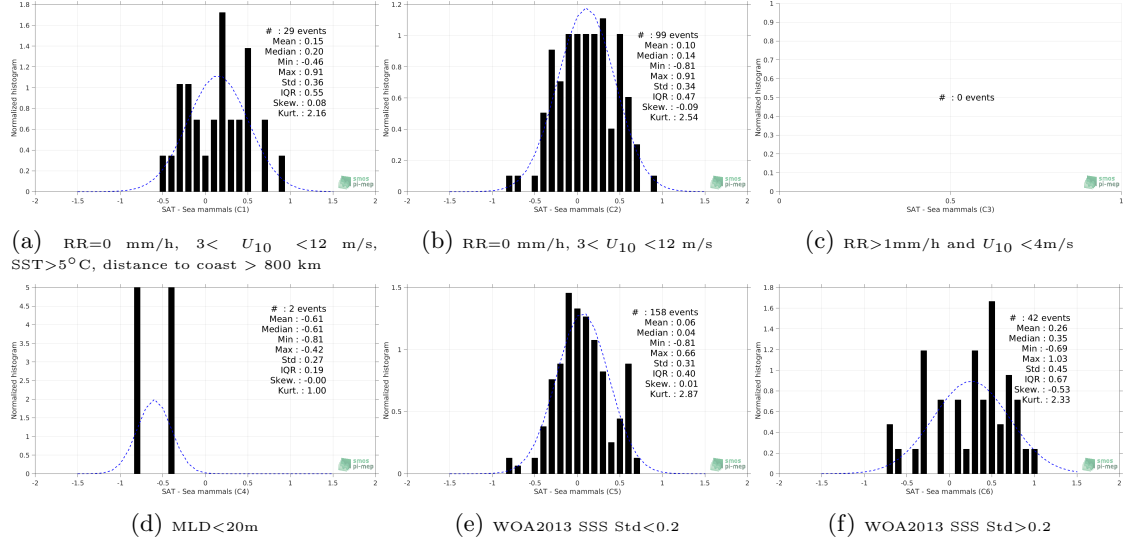
Figure 13: Normalized histogram of \Delta\text{SSS} (SMOS L3 v317 - Monthly - 25 km (CATDS-CPDC) - Sea mammals) for 6 different subdatasets corresponding to: RR=0 mm/h, 3 < U_{10} < 12 m/s, SST > 5^\circ\text{C} , distance to coast > 800 km (a), RR=0 mm/h, 3 < U_{10} < 12 m/s (b), RR > 1 mm/h and U_{10} < 4 m/s (c), MLD < 20 m (d), WOA2013 SSS Std < 0.2 (e), WOA2013 SSS Std > 0.2 (f).
