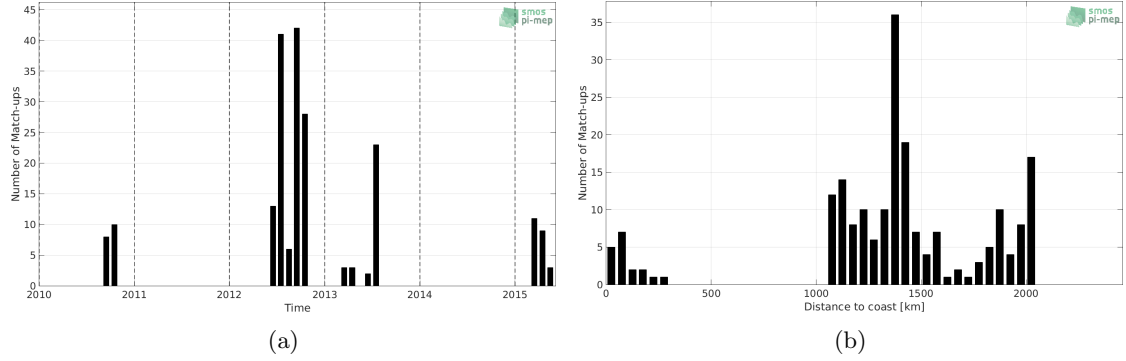
Figure 1: Number of match-ups between Sea mammals and SMOS L3 v317 - Monthly - 25 km (CATDS-CPDC) SSS as a function of time (a) and as function of the distance to coast (b) over the South Atlantic Ocean Pi-MEP region and for the full satellite product period.
