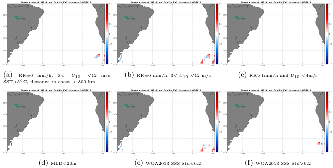
Figure 12: Temporal mean gridded over spatial boxes of size 1^{\circ}\times 1^{\circ} of \Delta\text{SSS} (SMOS L3 v317 - Monthly - 25 km (CATDS-CPDC) - Sea mammals) for 6 different subdatasets corresponding to: RR=0 mm/h, 3 < U_{10} < 12 m/s, SST >5^{\circ}\text{C} , distance to coast > 800 km (a), RR=0 mm/h, 3 < U_{10} < 12 m/s (b), RR >1 mm/h and U_{10} < 4 m/s (c),MLD <20 m (d),WOA2013 SSS Std <0.2 (e),WOA2013 SSS Std >0.2 (f).
