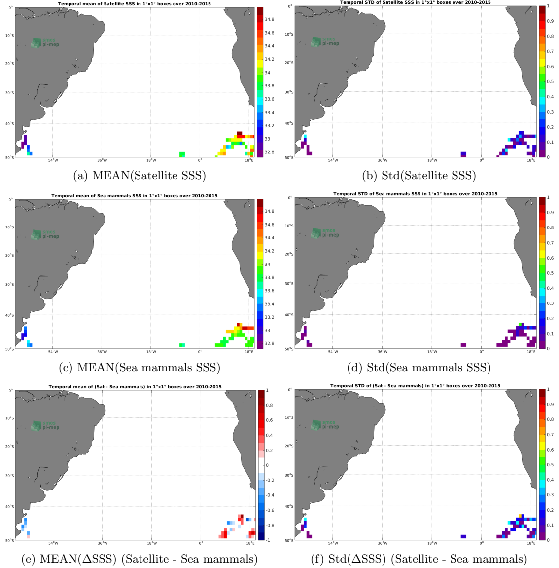
Figure 6: Temporal mean (left) and Std (right) of SSS from SMOS L3 v317 - Monthly - 25 km (CATDS-CPDC) (top), Sea mammals (middle), and of \Delta SSS (Satellite - Sea mammals). Only match-up pairs are used to generate these maps.
