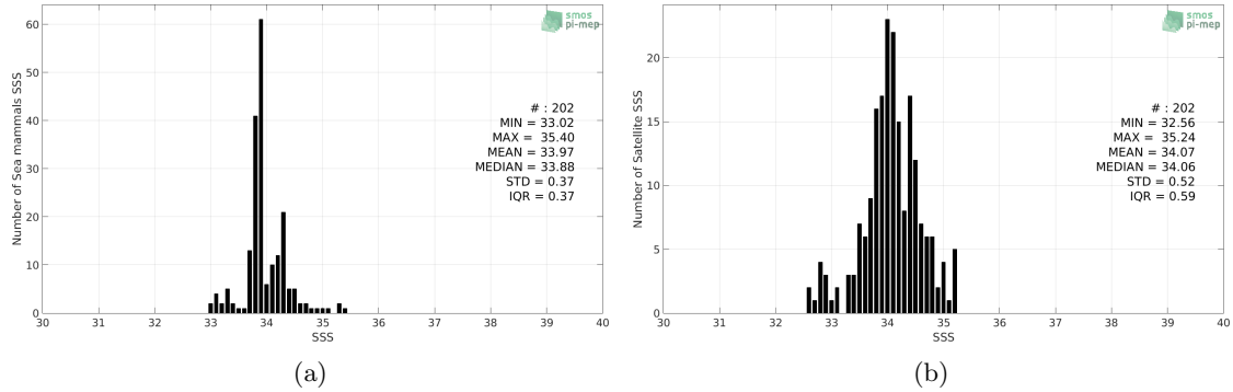
Figure 2: Histograms of SSS from Sea mammals (a) and SMOS L3 v317 - Monthly - 25 km (CATDS-CPDC) (b) considering all match-up pairs per bins of 0.1 over the South Atlantic Ocean Pi-MEP region and for the full satellite product period.
